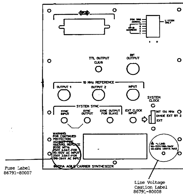
Figure 1. Label Location for 86791A Agile Carrier Synthesizer
