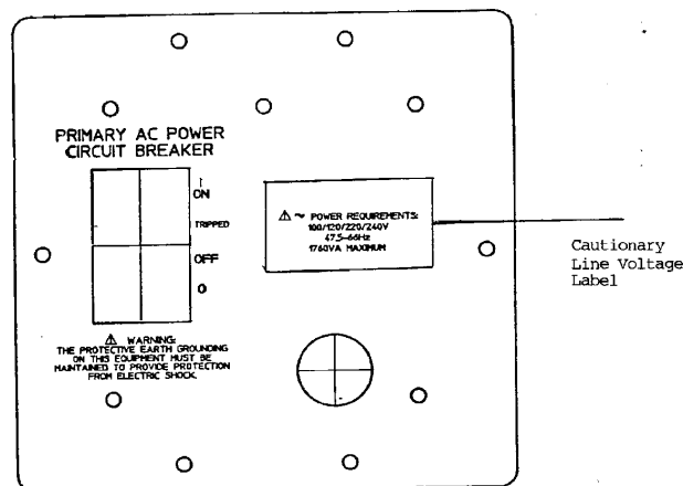
Figure 2. Rear Door Cautionary Line Voltage Label Location
