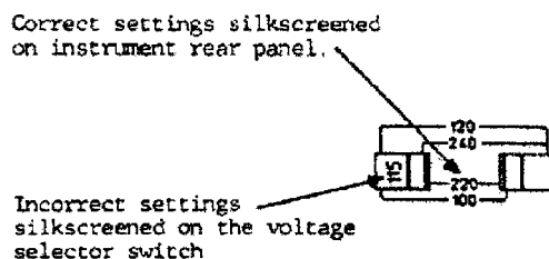
Figure 1. AC Line Voltage Switch Positions
