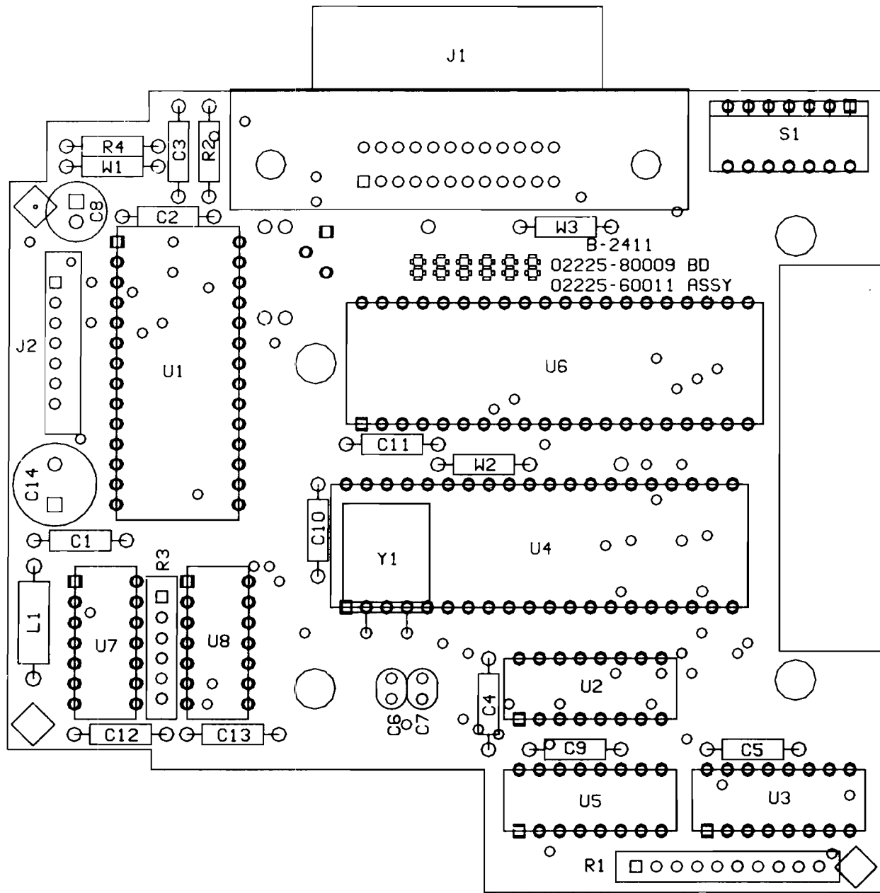
Figure 9-3. 02225-60011 Assembly Drawing
