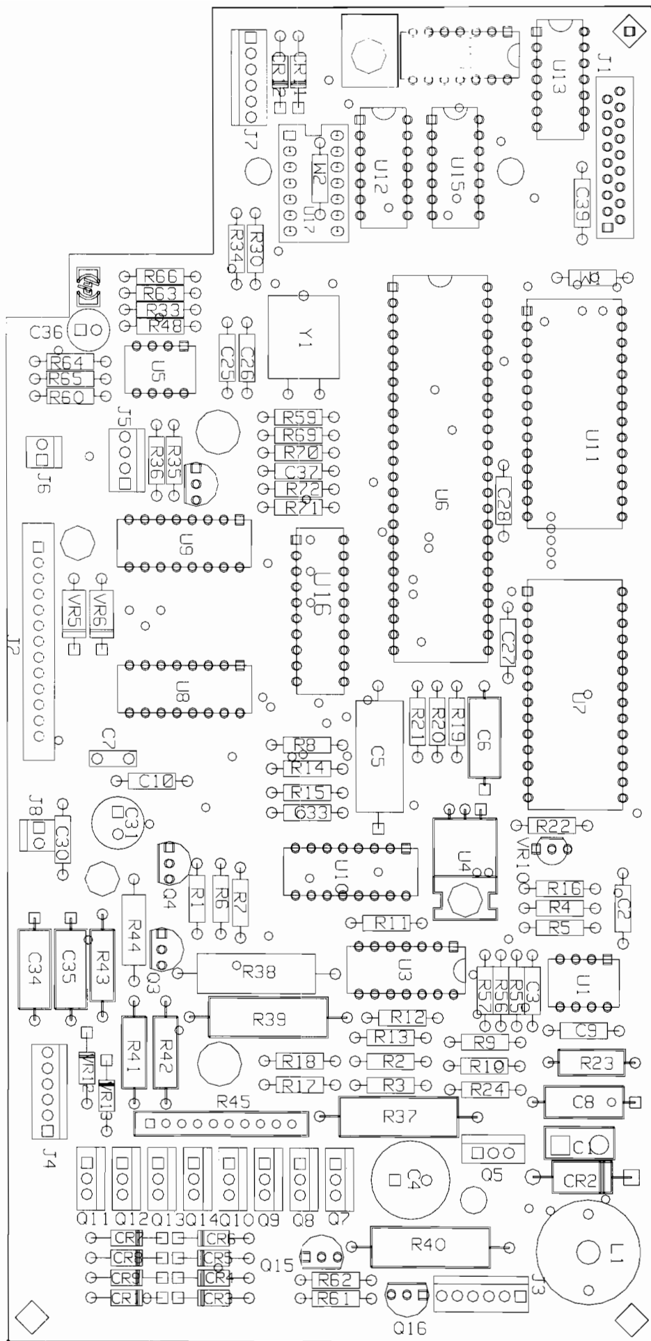
Figure 9-12. HP 2225P Main Logic PCA Assembly Drawing
