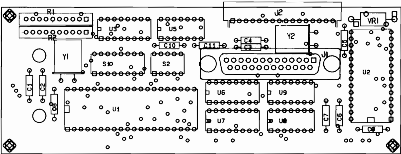
Figure 12-12. 02225-60019 Assembly Drawing
