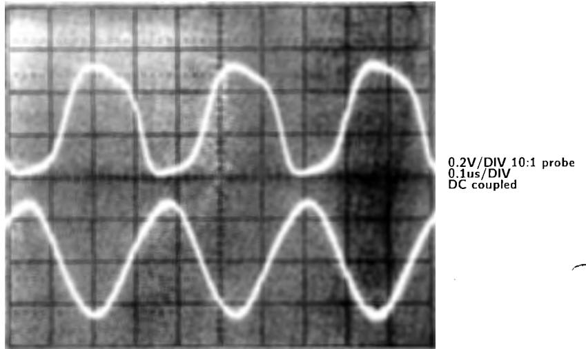
Figure 8-2. Crystal Waveform
