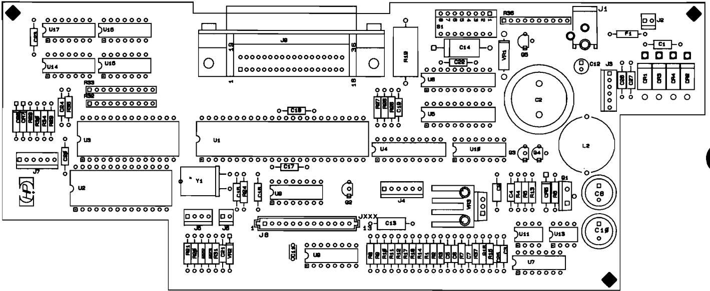
Figure 12-8. 02225-60072 Assembly Drawing
