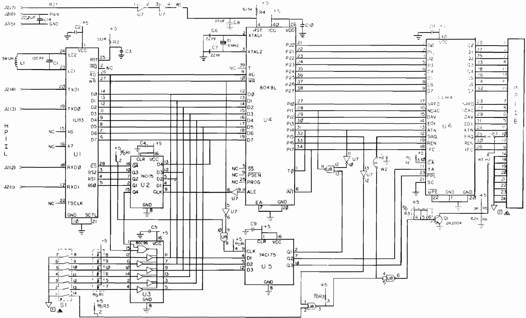
Figure 12-5. 02225-60011 Schematic
