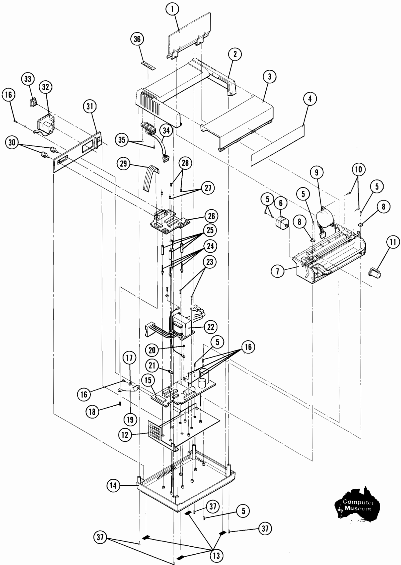
Figure 9-1. HP 2225A ThinkJet Printer Overall View
