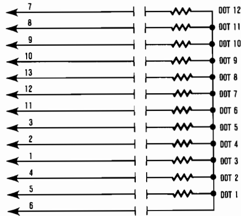
Carriage Assembly Print Head
