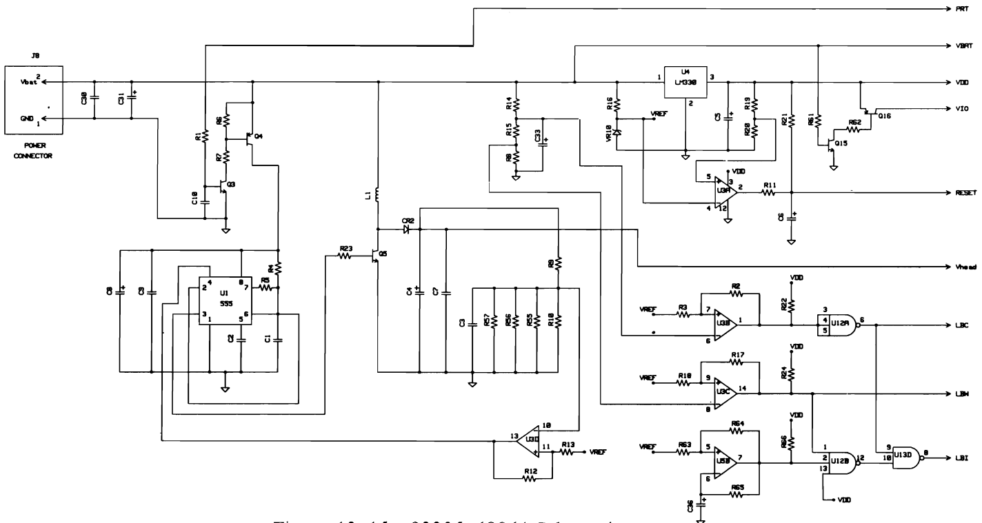
Figure 12-15. 02225-60061 Schematic (1 of 2)
