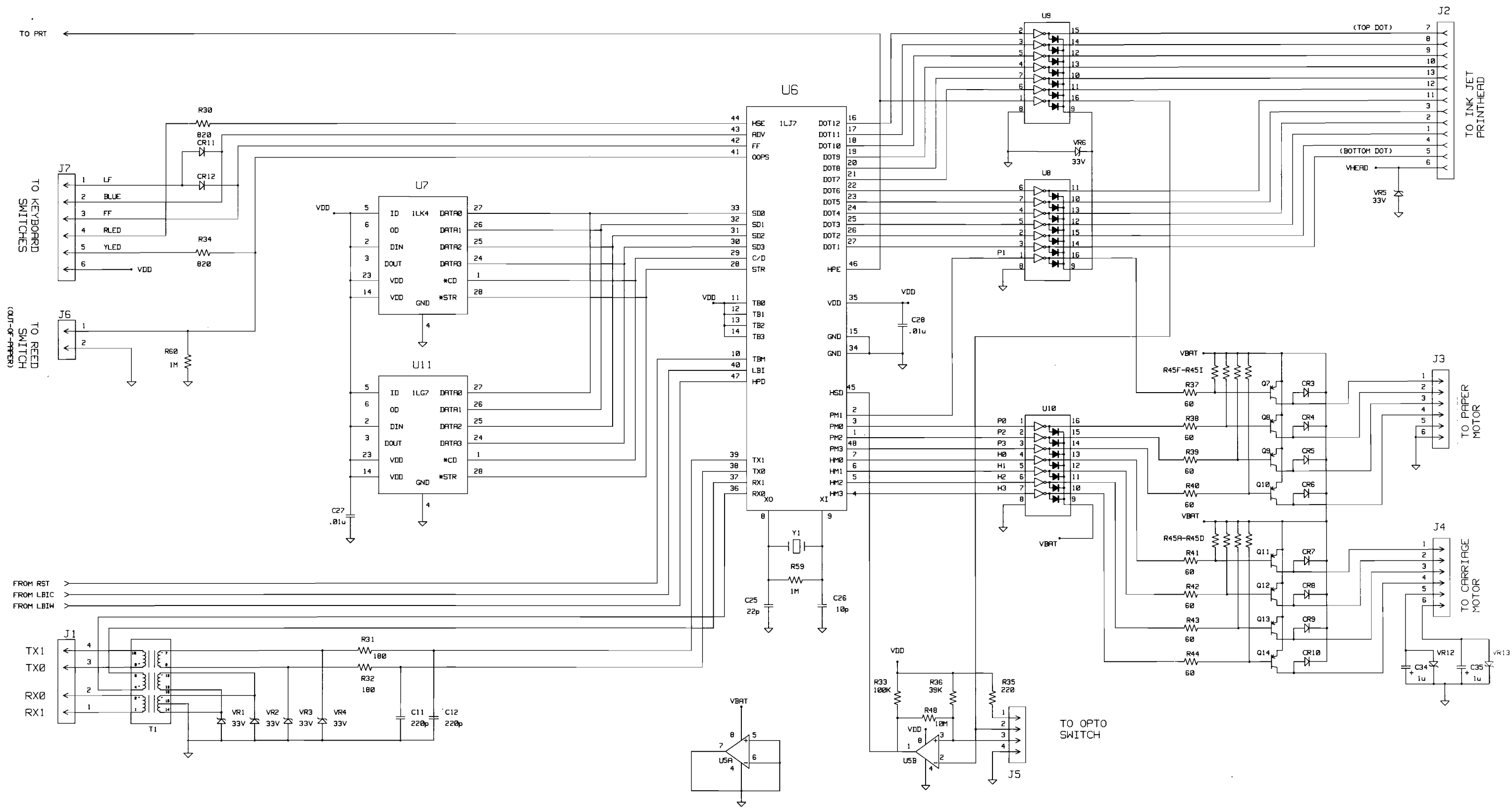
Figure 12-7. 02225-60001 Schematic (2 of 2)
