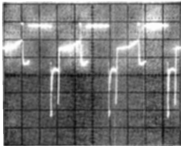
Figure 8-5. 2225B/P at Connector J4 Pins 1-4
