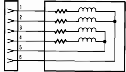
Motor Assembly
