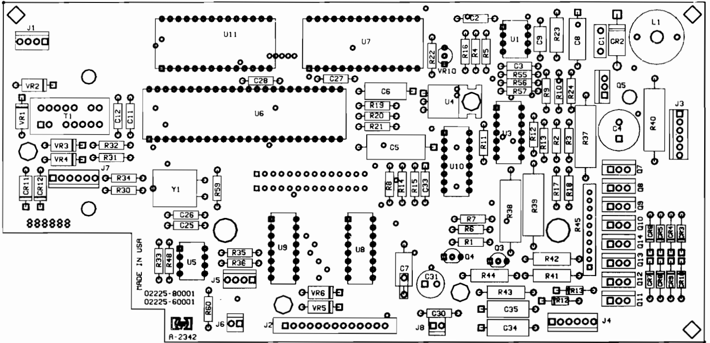
Figure 12-6. 02225-60001 Assembly Drawing
