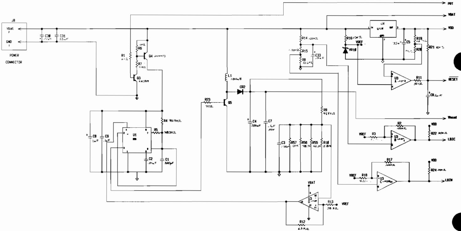
Figure 12-7. 02225-60001 Schematic (1 of 2)
