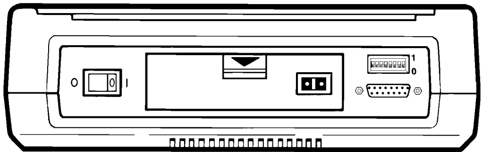
Figure 1-8. HP 2225P Rear View
