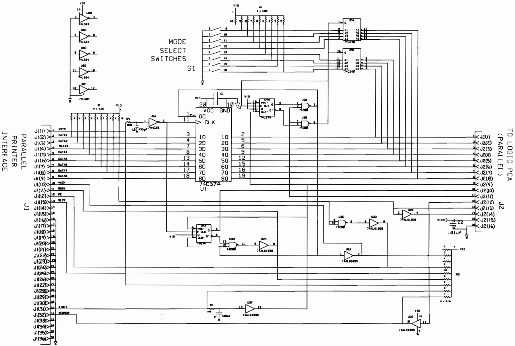
Figure 11-10. Earlier Version 2225C I/O PCA Schematic
