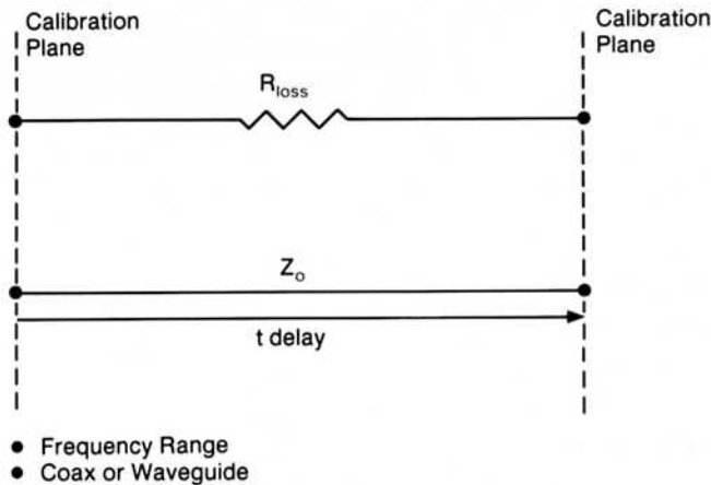
Model for Transmission Standard (Thru)
