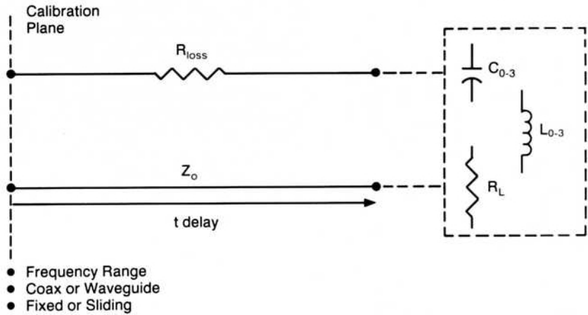
Model for Reflection Standard (Short, Open, Load or Arbitrary Impedance)
