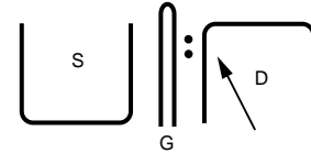
Figure 2. Typical Location of ESD damage in FETs
