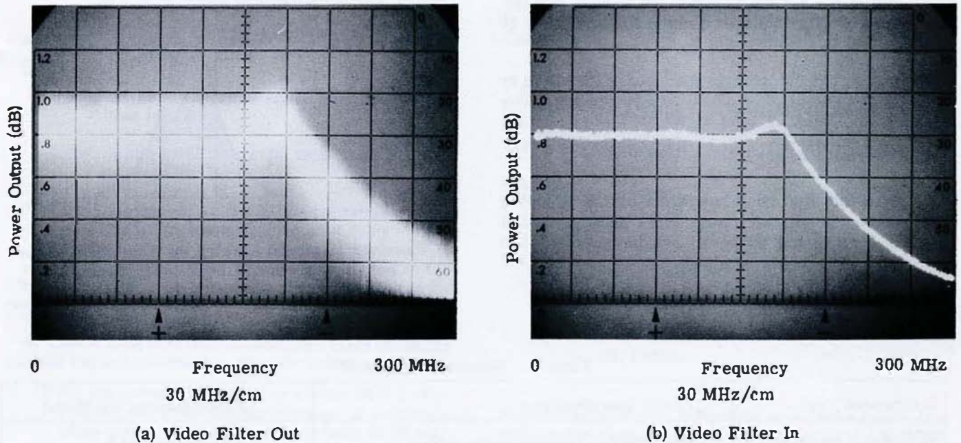
Figure 3. Noise Output of a Broadband Amplifier Showing the Effect of the Video Filter.
