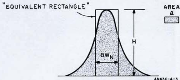
Figure 4 Receiver Passband Showing the Equivalent Noise Rectangle from which the Noise Bandwidth is Calculated.
