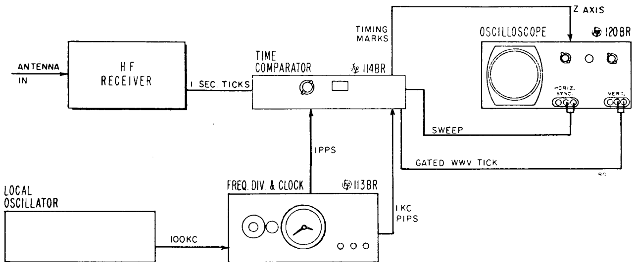
METHOD B. Simplified Time Comparison without Shifting Phase of Local Ticks
