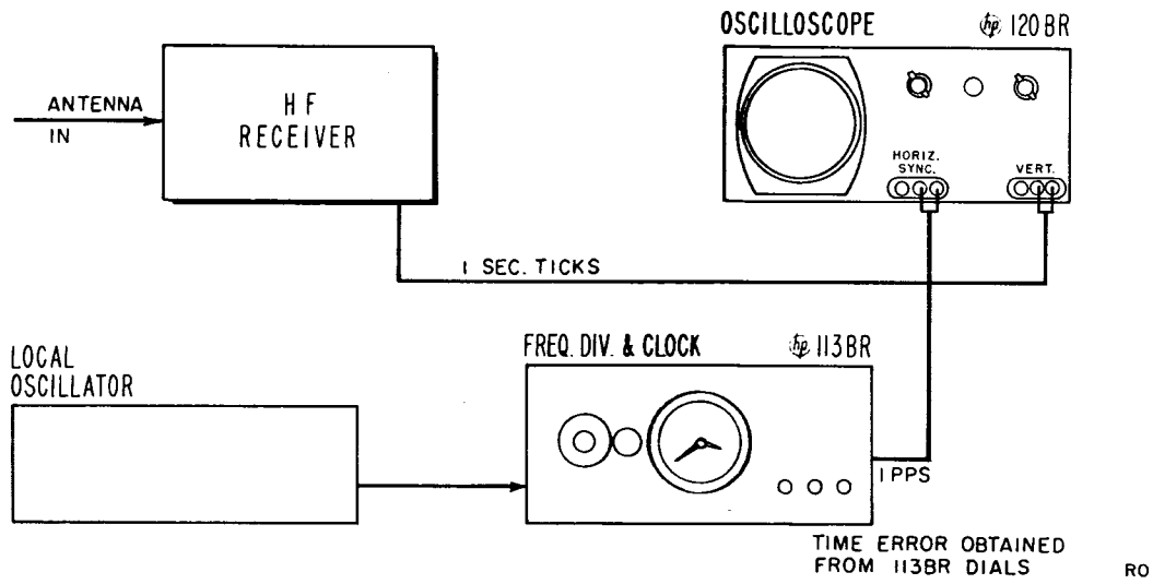
METHOD A. Requires Adjustment of Model 113BR Tick Phasing
