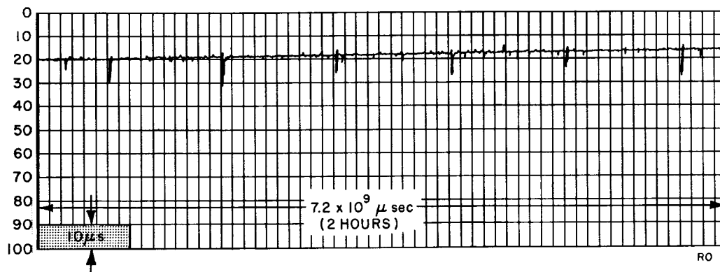
Figure 3-5. Strip-Chart Recording of VLF Frequency Comparison Using WWVL Over Two Hour Period
