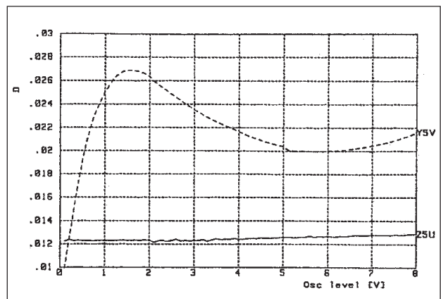
Figure 4. Signal Voltage Dependence of Loss Coefficient
