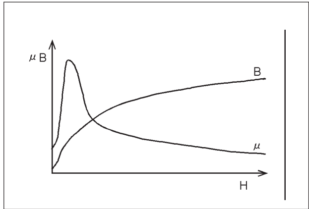
Figure 6. Magnetic Characteristics
