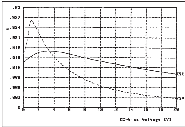
Figure 2. Loss Coefficient of DC Bias Dependence
