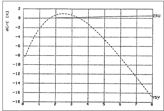
Figure 3. Signal Voltage Dependence of Capacitance
