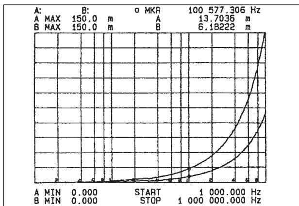
Figure 5. Frequency Characteristics of Loss coefficient of Film Capacitors (by the HP 4194A)
