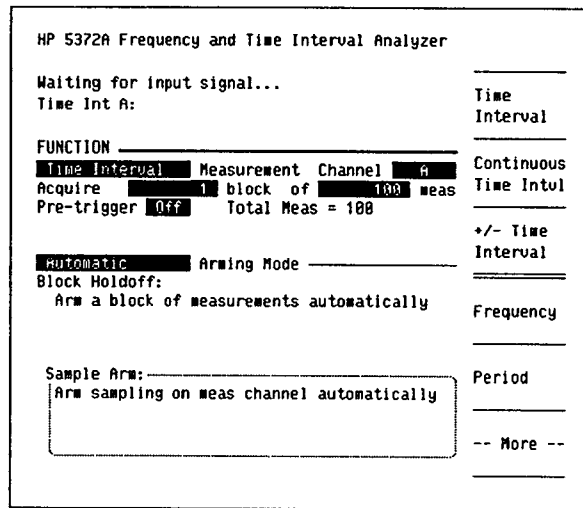
Figure 4. HP 5372A display screen after pushing the Preset key.
