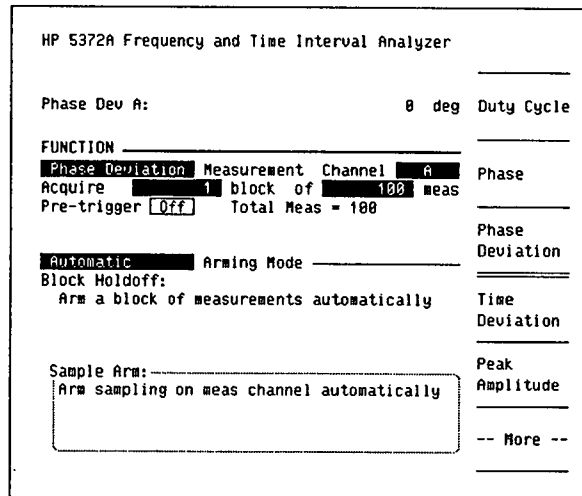
Figure 5. Select a Phase Deviation measurement on the FUNCTION menu.
