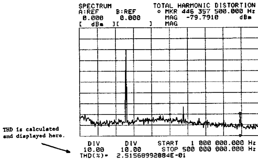
Figure 6. The Total Harmonic Distortion
