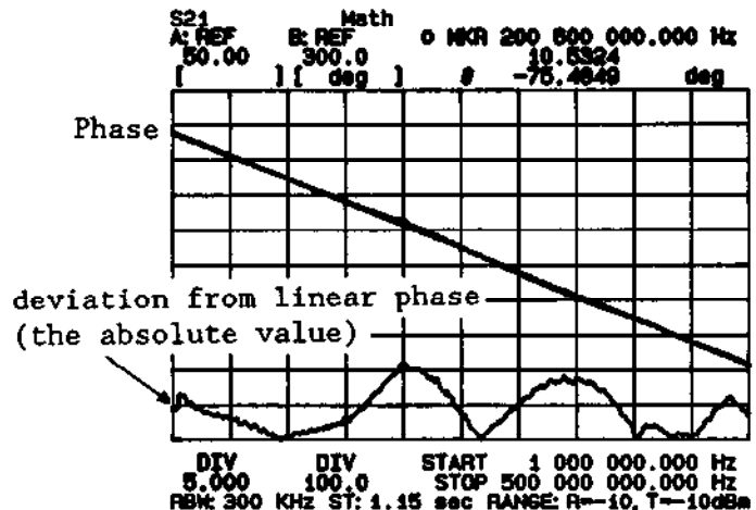
(B) The Deviation from Linear Phase
