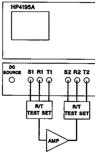
Figure 2. The S-parameter Measurement Configuration
