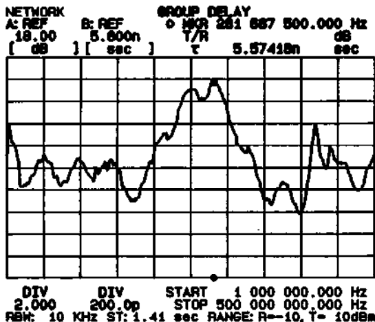
(A) The Group Delay
