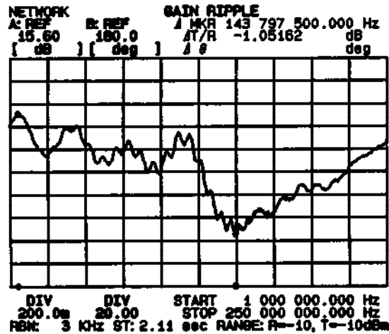
Figure 4. The Gain Ripple
