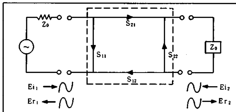
Figure 1. The S-parameter Concept
