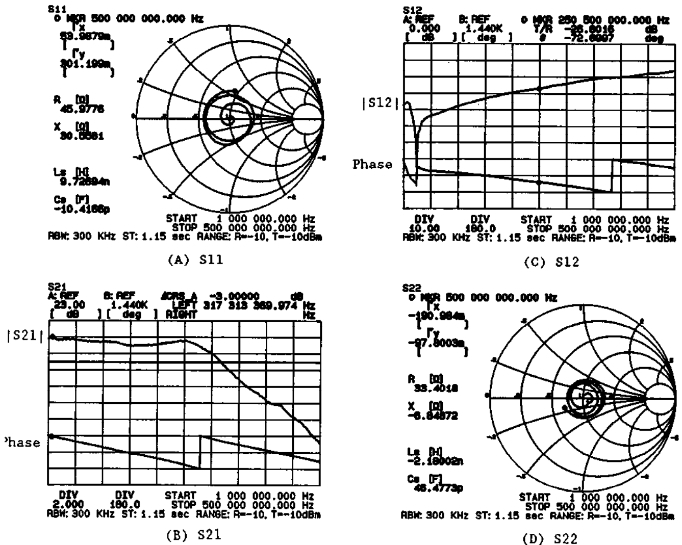
Figure 3. The S-parameter
