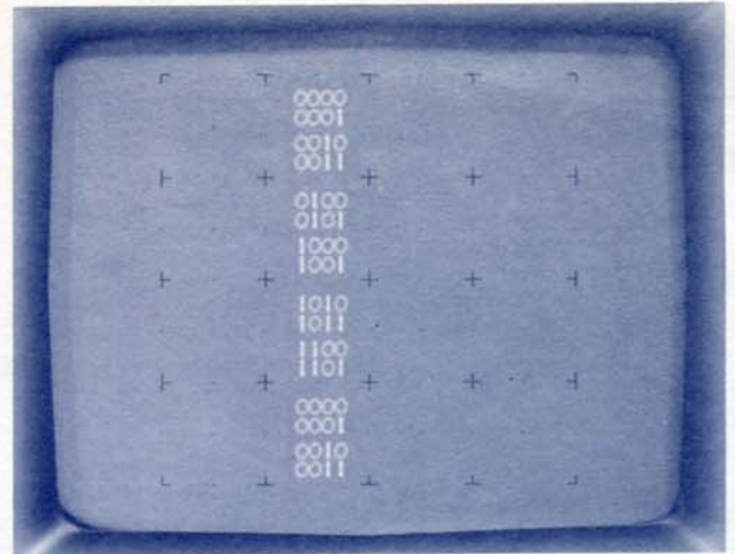
3. Data-domain count. The output of a counter can be examined easily if it is displayed as binary digits.
