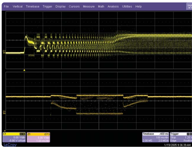
Figure 8. Start-up motor drive signal capture using a LeCroy WaveSurfer scope
