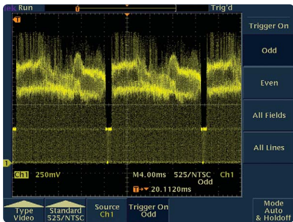
Figure 5. Full frame of composite video using the Tektronix TDS3000 Series DPO scope
