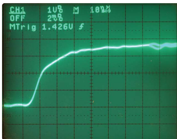
Figure 14. The analog oscilloscope fails to show the infrequent glitch
