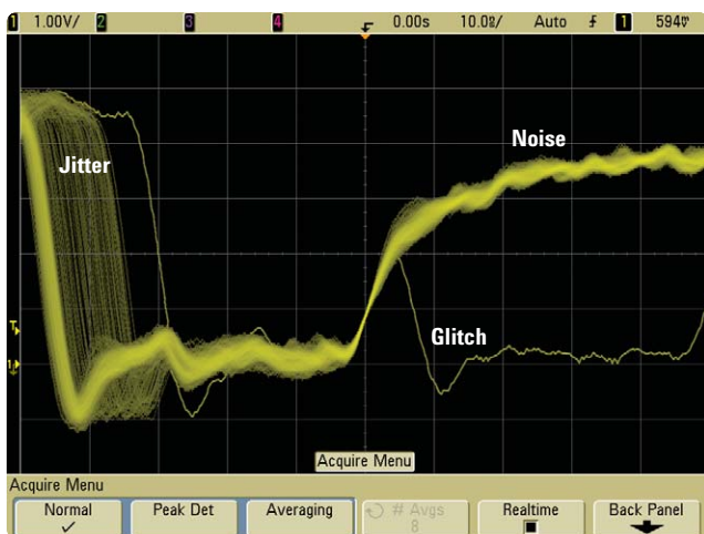
Figure 13. Display intensity gradation shows characteristics of jitter, noise, and signal anomalies on Agilent's 6000 Series oscilloscope
