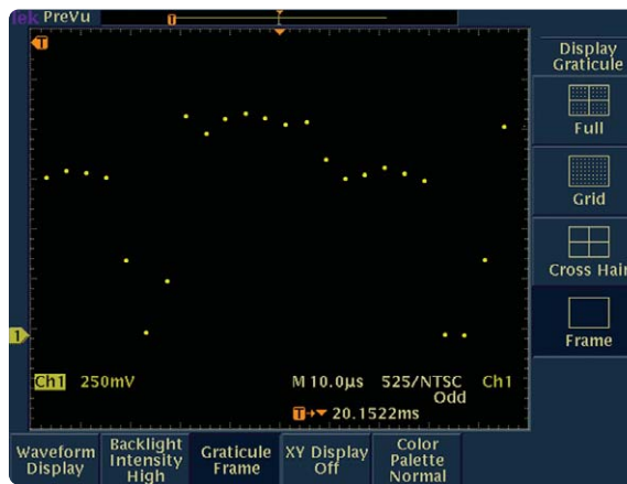
Figure 6. Zoomed-in display of a single line of video using the Tek TDS3000 Series scope (note: dots have been enhanced for clarity)
