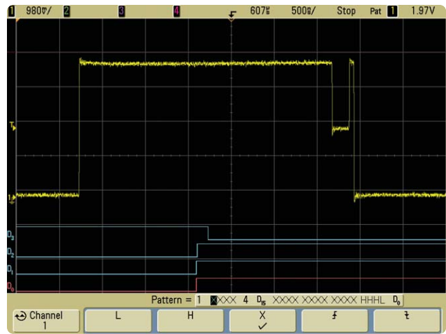
Figure 10. Zooming-in on a “bright spot” reveals a runt pulse
