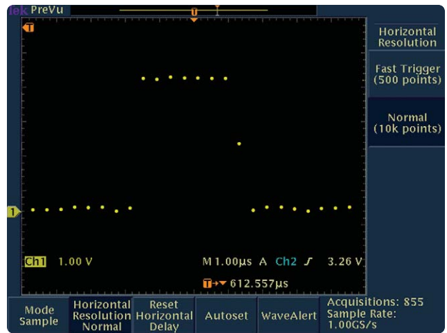
Figure 12. Zooming-in on the burst shows just a single digitized point on the runt pulse due to insufficient sample rate and memory depth (note: dots have been enhanced for clarity)
