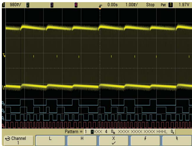
Figure 9. Agilent 6000 Series scope reveals “bright spots” buried within each digital burst
