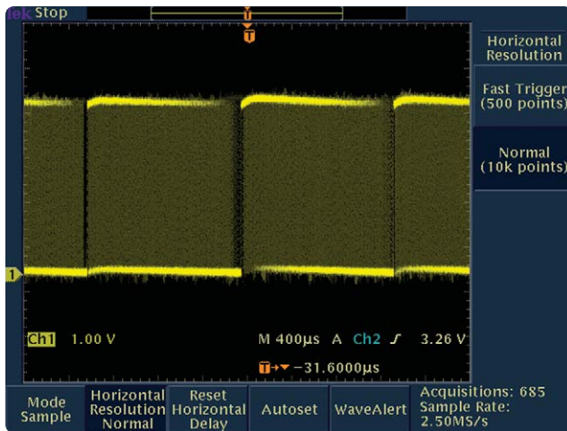
Figure 11. The Tek TDS3000 Series scope fails to reveal any embedded "bright spots"
