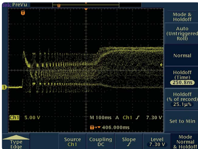
Figure 8. Start-up motor drive signal captured using a Tektronix TDS3000 Series scope
