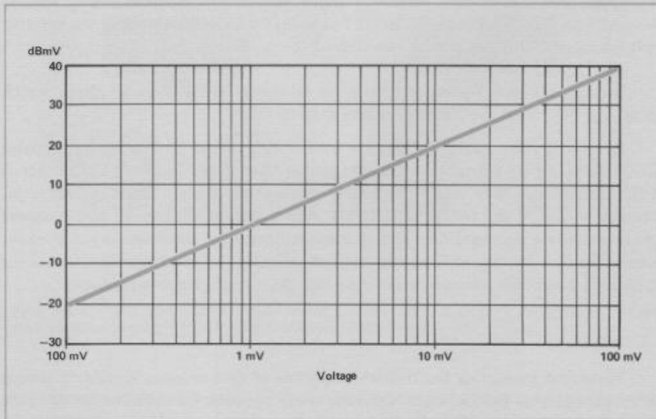
Figure 3-6. Conversion from dBmV to voltage (either 50 \Omega or 75 \Omega ). For voltage levels outside the chart remember that for every 20 dBmV change the voltage changes by a factor of 10. Example: -105 dBmV is -5 dBmV with a 100 dB change. From the chart, -5 dBmV = 560 \mu V, and -100 dB is a change of \times 10^{-5} . Therefore, -105 dBmV = 560 \times 10^{-5} \mu V = 5.6 \times 10^{-9} V.
