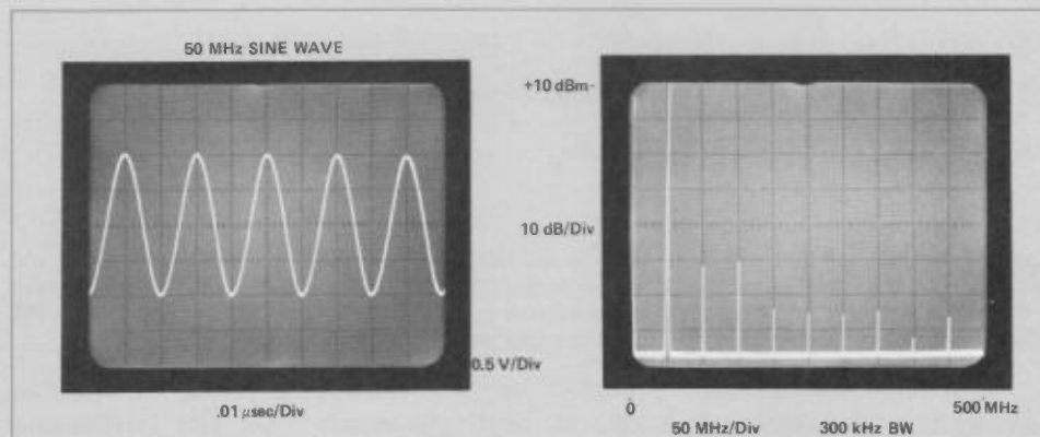
Figure 1-3. The photo at the left shows a 50 MHz sine wave in the time domain. The photo at the right shows the frequency domain which illustrates distortion components spaced 50 MHz apart.
