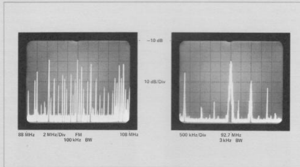
Figure 2-1. The FM broadcast frequency spectrum at Palo Alto, California, is shown in the photo at the left. Identification of a 92.7 MHz signal in the FM broadcast band is shown in the photo at the right.
