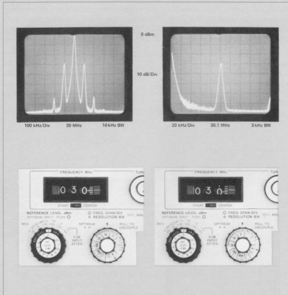
Figure 3-3. A 30-MHz signal frequency modulated by a 100-kHz signal is shown in the left photo. The right photo identifies the frequency of the first-order upper sideband as 30.1 MHz.
