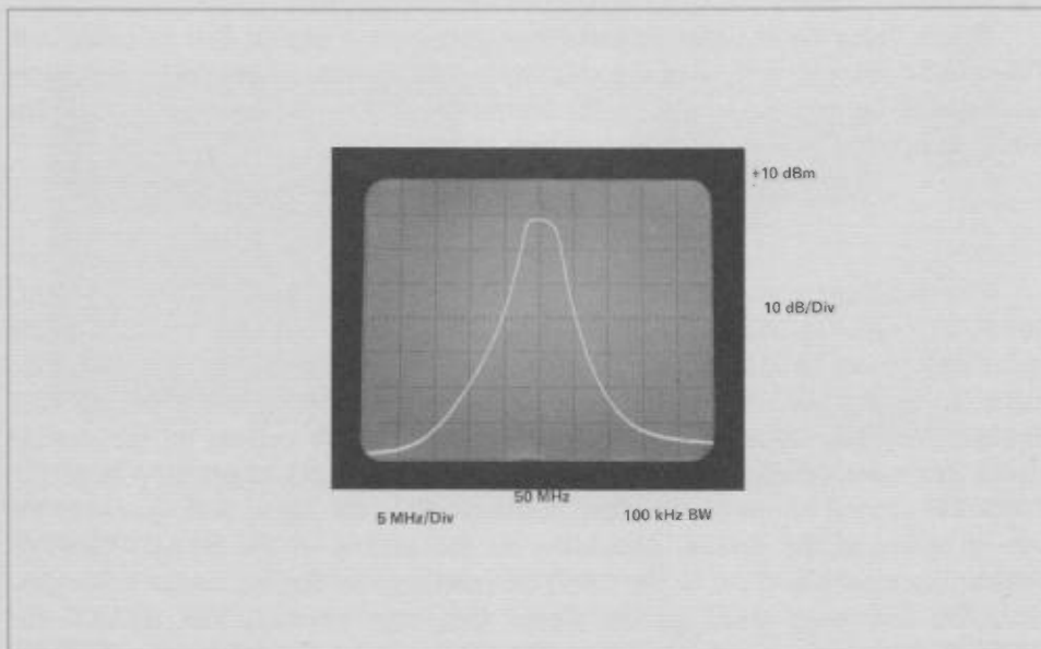
Figure 2-6. Insertion loss of a 50 MHz BPF using the 8444A-058 Tracking Generator.
