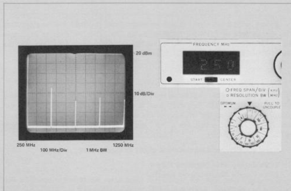
Figure 4-2. Harmonic distortion of a 250 MHz signal.
