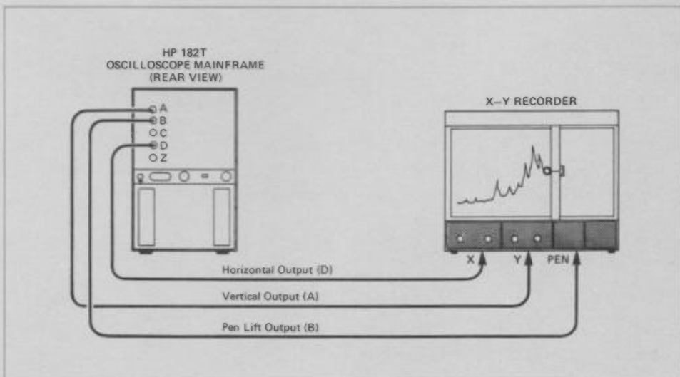
Figure C-2. Using 182T to connect an X-Y recorder to the 8558B Spectrum Analyzer.
