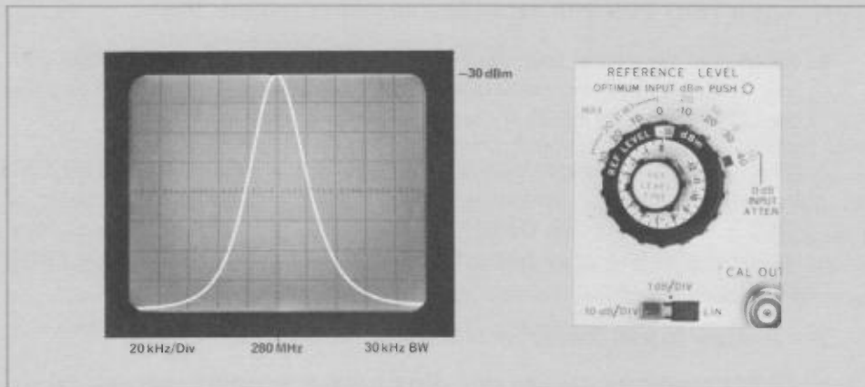
Figure 6-2. To calibrate the reference level, set the vertical scale for LIN and set the peak of the CAL signal on the reference level with the REF LEVEL CAL adjust.
