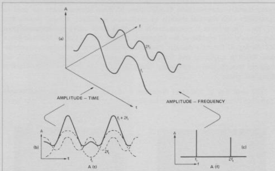
Figure 1-1. The time and frequency domains: (a) Three-dimensional coordinates showing time, frequency, and amplitude. The addition of a fundamental and its second harmonic is shown as an example. (b) View seen in the A(t) plane. On an oscilloscope, only the composite f_1 + 2f_1 would be seen. (c) View seen in the A(f) plane. Note how the components of the composite signal are clearly seen here.
