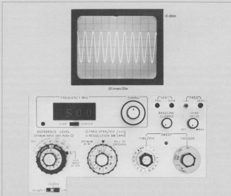
Figure 5-3. The 0 kHz/DIV setting on the 8558B Spectrum Analyzer used for a time domain view of a 500 MHz signal with 50% AM and 100 kHz modulation frequency.
