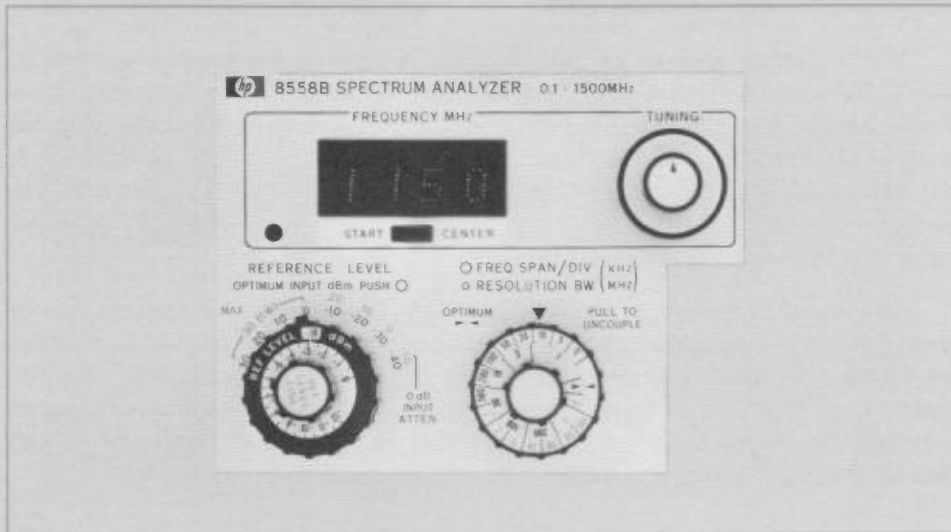
Figure 4-1. Three knob settings for simple operation.
