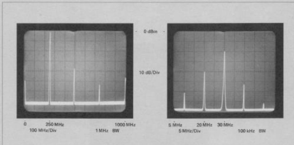
Figure 2-2. A 250 MHz signal with harmonic distortion components at 500, 750, and 1000 MHz is shown at the left. The right photo shows two input signals at 20 MHz and 30 MHz with resulting intermodulation distortion at 10, 40, and 50 MHz.
