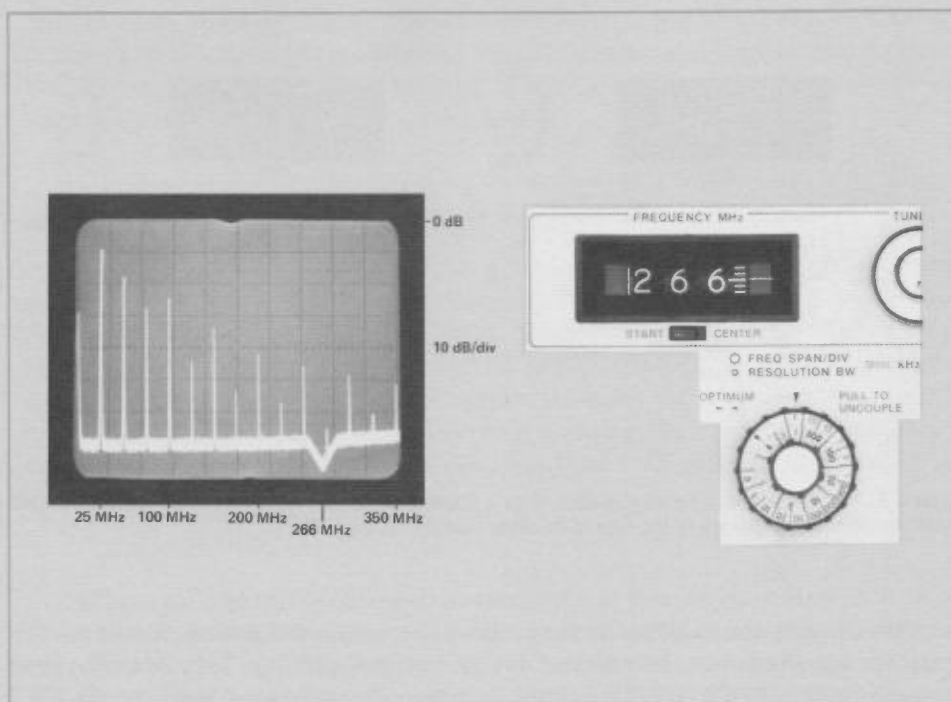
Figure 3-2. Harmonic distortion of a 25 MHz signal. In the full scan mode, the frequency readout corresponds to the position of the CRT marker notch.
