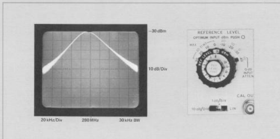
Figure 6-1. To calibrate the vertical scale for 10 dB/DIV, set the vertical scale for 10 dB/DIV and set the peak of the CAL signal on the reference level with the VERT GAIN adjust.
