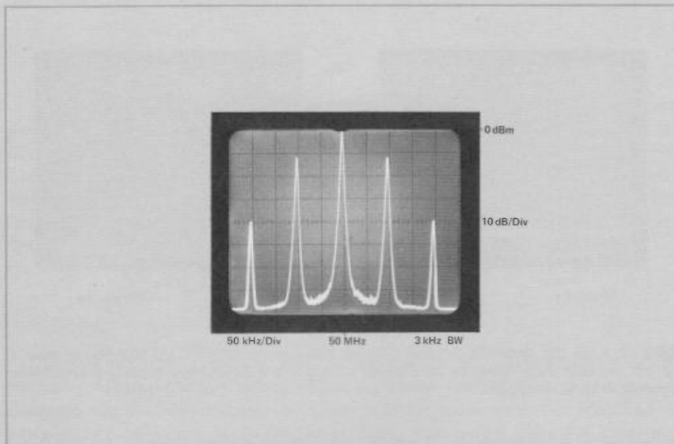
Figure 2-4. Frequency domain of a 50 MHz signal with 50% AM and 4% second harmonic distortion.
