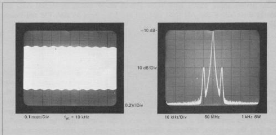
Figure 2-3. The left photograph is a time domain view of a 50 MHz signal with 2% AM. The carrier frequency, sideband levels (% modulation and distortion), and modulation frequency are easily measured in the frequency domain shown in the right photograph.
