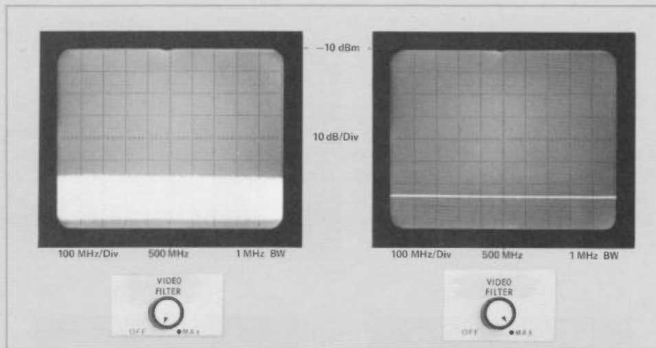
Figure 5-2. Noise averaging effect of the VIDEO FILTER MAX position.
