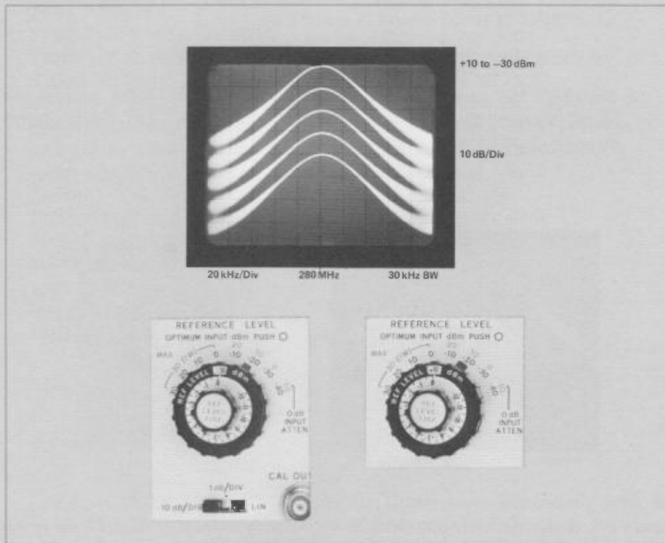
Figure 6-3. To check the 10 dB/DIV calibration of the vertical scale, change REF LEVEL dBm in 10 dB steps and see if the trace moves one division for each 10 dB change.
