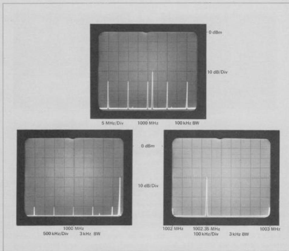
Figure 5-6. The 8406A Frequency Comb Generator is used to improve the accuracy of frequency determination. In the photo at the top, a 10 MHz comb is used to reference the unknown signal. In the left photo, the comb is reduced to 1 MHz for greater accuracy. In the photo at the right, the frequency span is reduced and the frequency of the unknown signal is determined (1002.35 MHz \pm 117 kHz). Accuracy is \pm 0.01% of reading \pm 5% of frequency separation between nearest comb tooth and signal to be measured.
