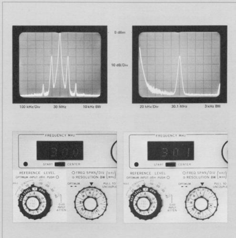
Figure 4-3. A 30 MHz signal frequency modulated by a 100 kHz signal is shown in the left photo. The right photo identifies the frequency of the first-order upper sideband as 30.1 MHz.
