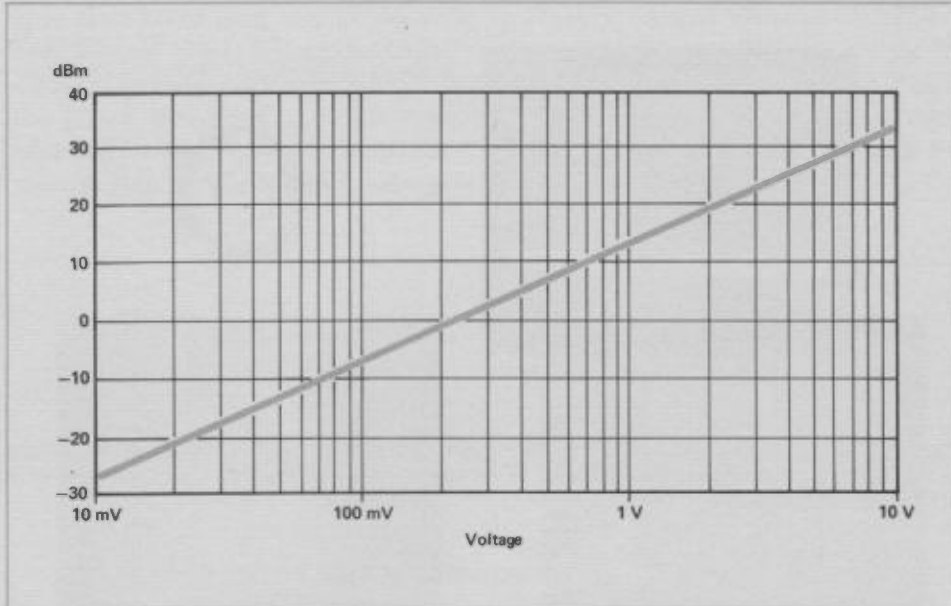
Figure 3-5. Conversion from dBm to voltage in 50 \Omega . For power levels outside this chart remember that a 20 dB change in power means a factor of 10 change in voltage. Example: -63 dBm is -3 dBm with a 60 dB change. From the chart, -3 dBm = 160 mV and -60 dB is a voltage change of \times 10^{-3} . Therefore, -63 dBm = 160 \times 10^{-3} mV = 160 \mu V.
