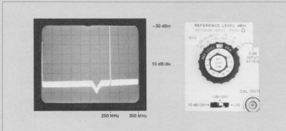
Figure 3-4. Relationship between REFERENCE LEVEL control and reference level on the CRT. When operating in the FULL scan mode, the marker notch must be far enough away from the signal to be measured so as not to be affect its amplitude.
