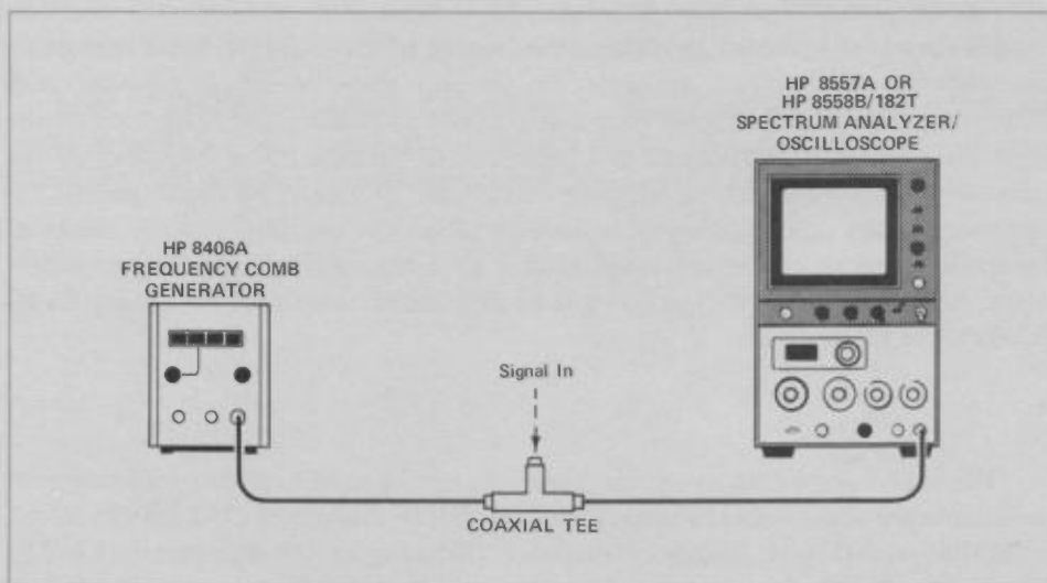
Figure 5-5. Block diagram of instruments used to make accurate frequency measurements.
