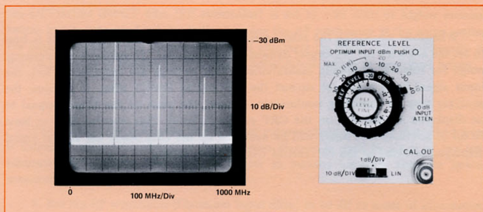
Figure 3-4. Relationship between REFERENCE LEVEL control and reference level on CRT.
