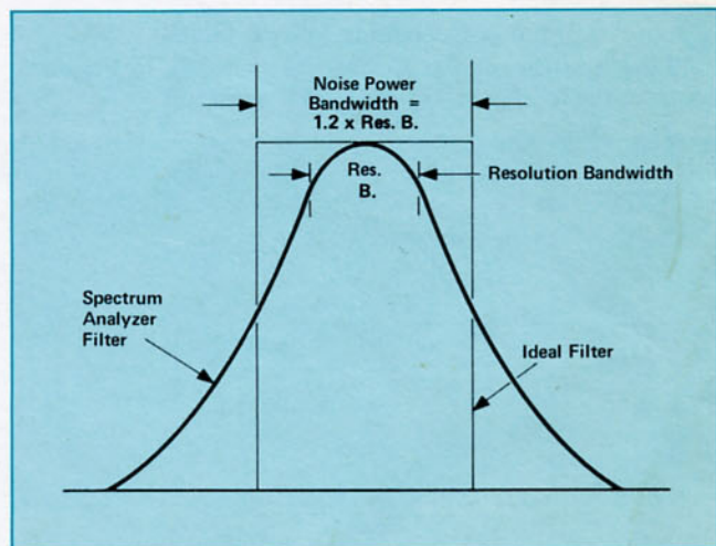
Figure 2. Comparison of Real & Ideal Filter Response showing the Equivalent Noise Power Bandwidth.
