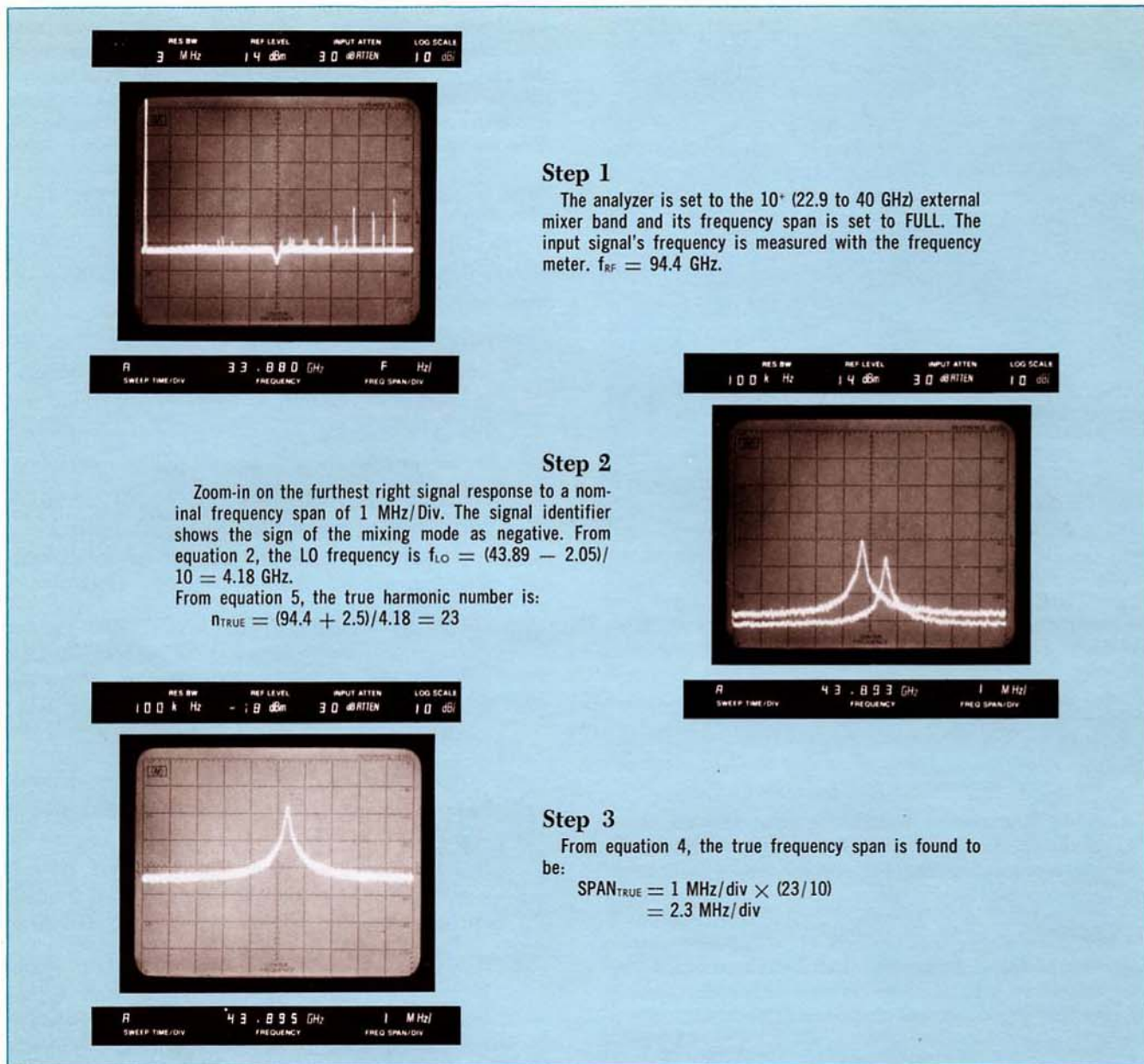
Figure 4. Measurement Example.
