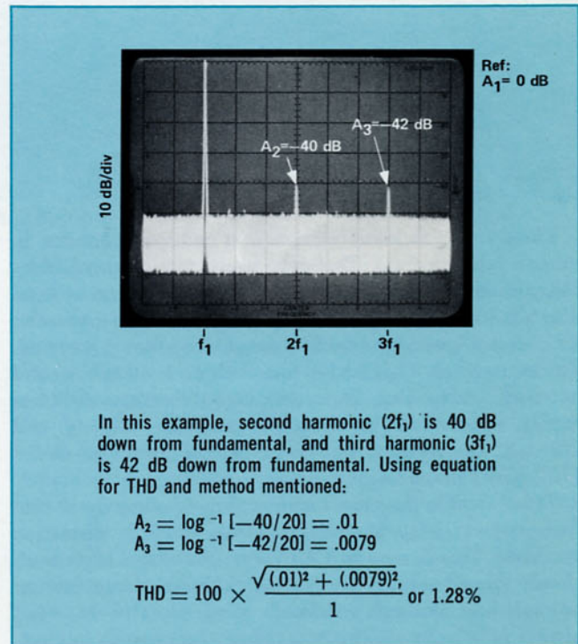
Figure 1. Harmonic Distortion.
