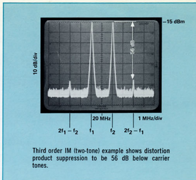
Figure 3. Two-Tone Third-Order IM.
