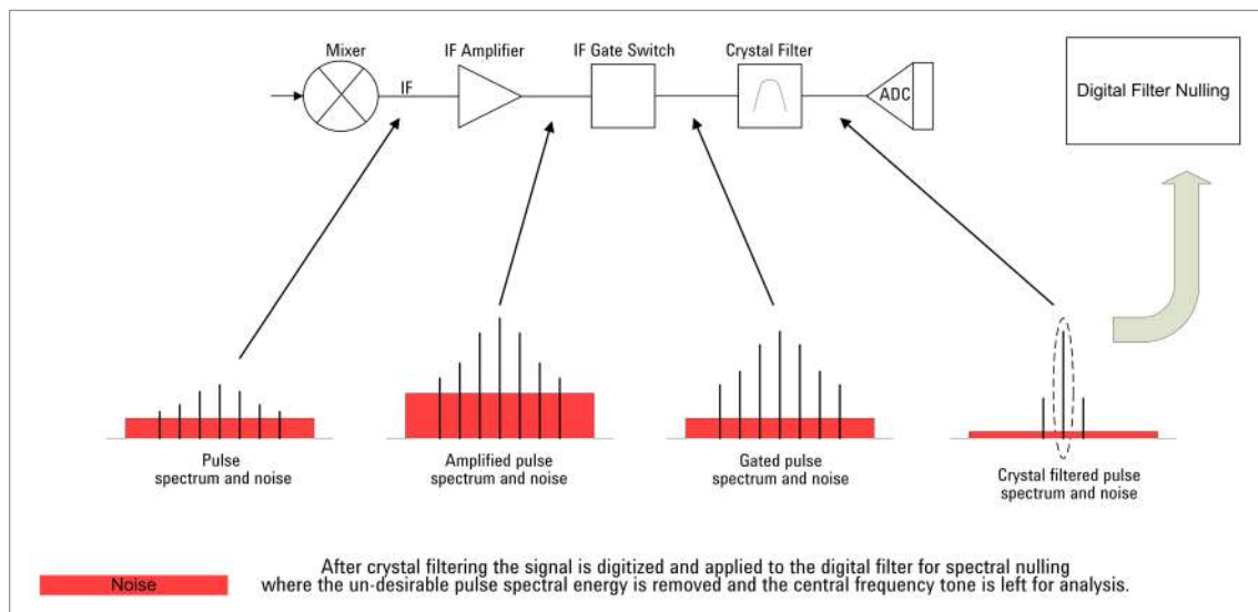
Figure 17. Narrowband filter path
