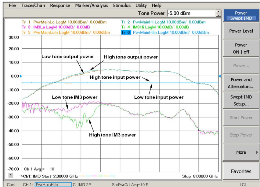
Figure 30b. Wideband pulse swept-frequency IMD measurements with receiver leveling
