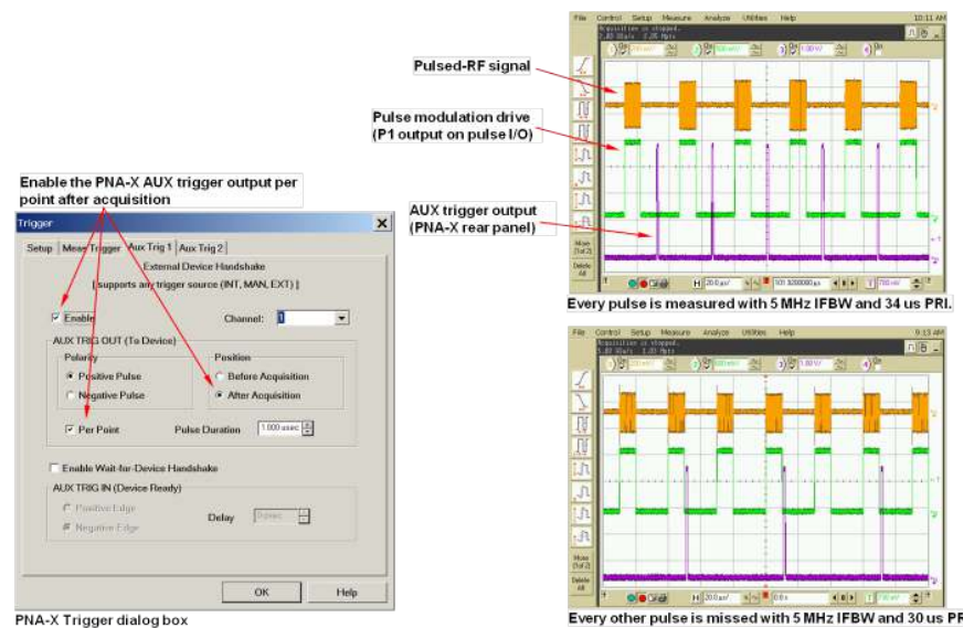
Figure 15. Wideband pulse-to-pulse measurement verification
