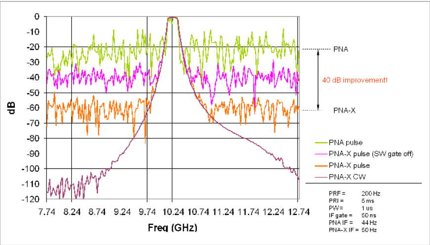
Figure 20. System dynamic range comparisons, 40 dB improvement with PNA-X and software gating
