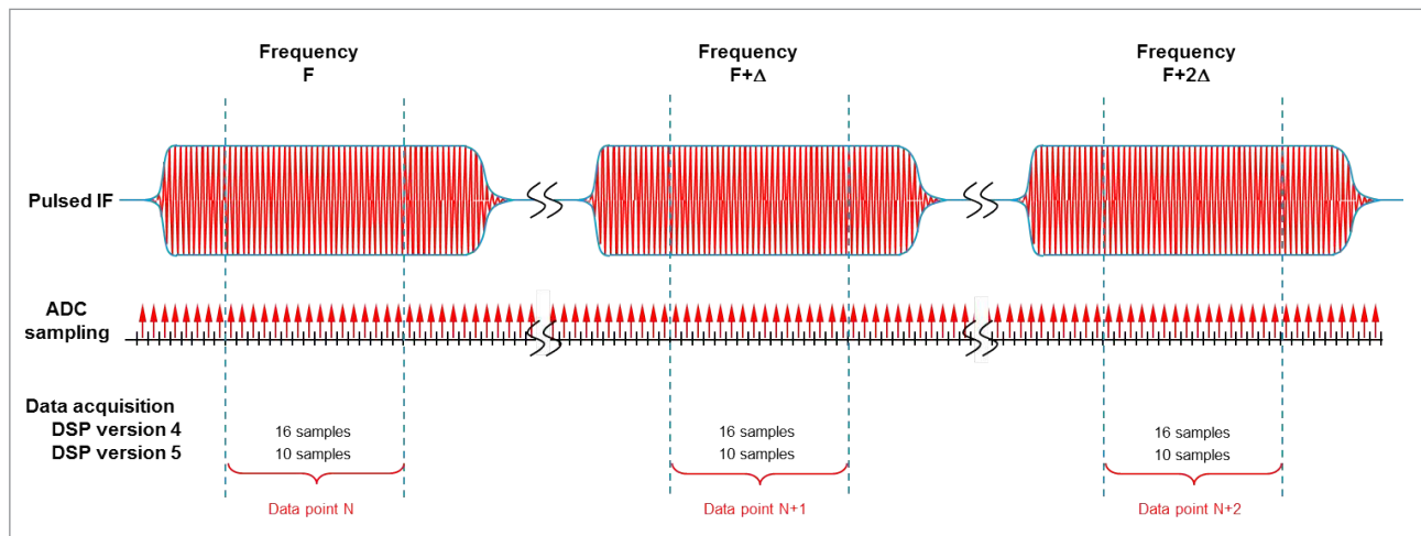
Figure 12. Wideband point-in-pulse and pulse-to-pulse data acquisition with widest IF bandwidth
