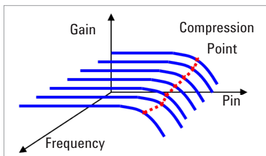
Figure 28. Compression measurements vs. frequency
