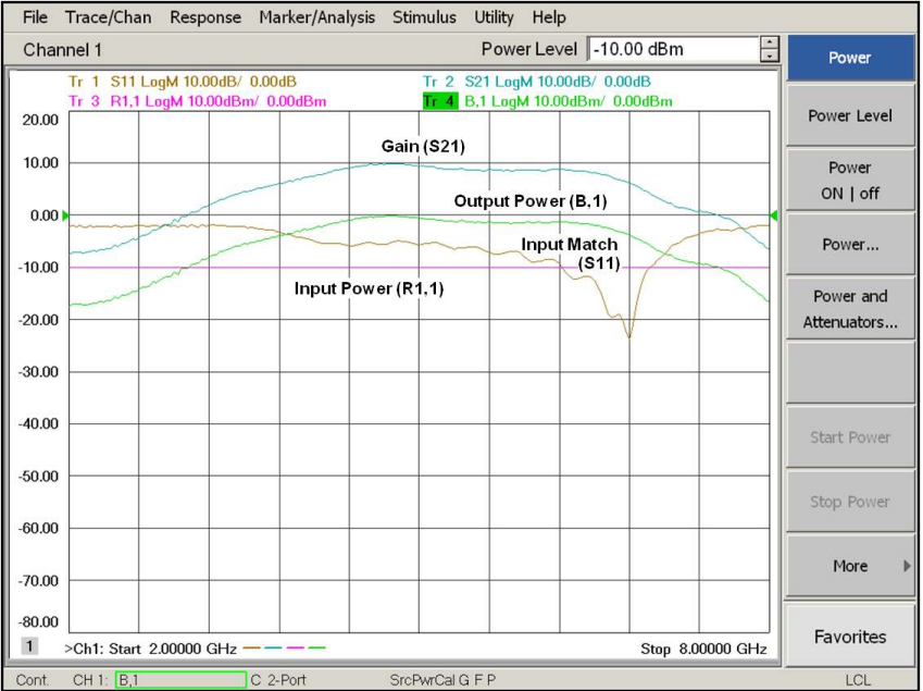
Figure 25c. Corrected pulsed-RF S-parameters and absolute power measurements using narrowband detection
