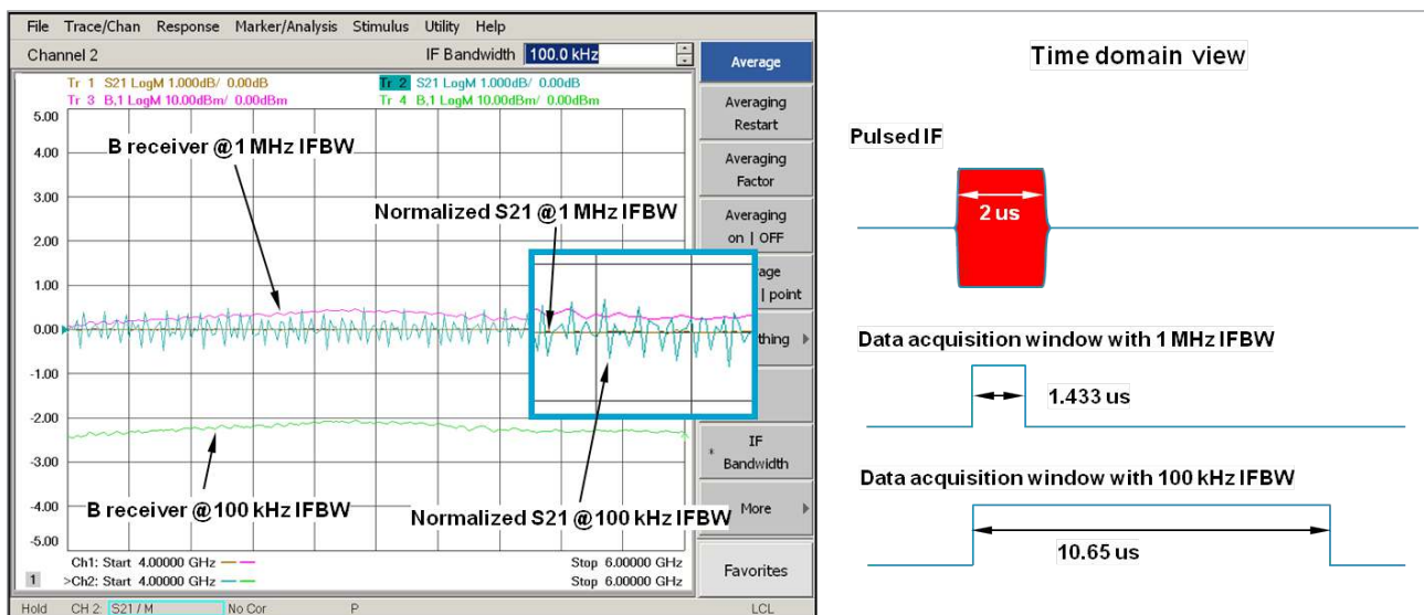
Figure 14a. Measurement errors caused by improper IF bandwidth
