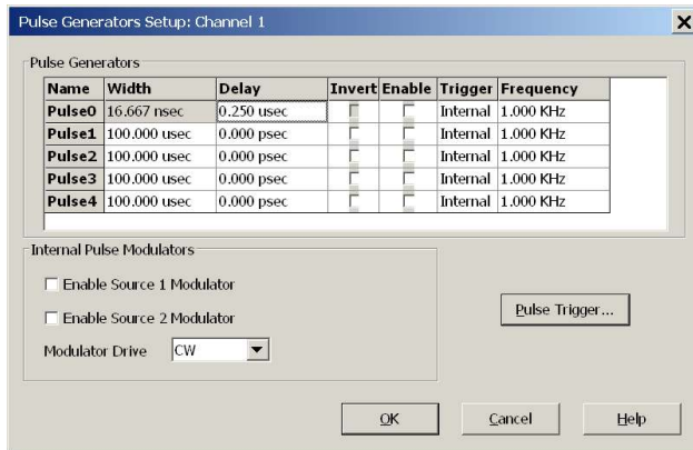
Figure 10a. Pulse Generators Setup dialog box
