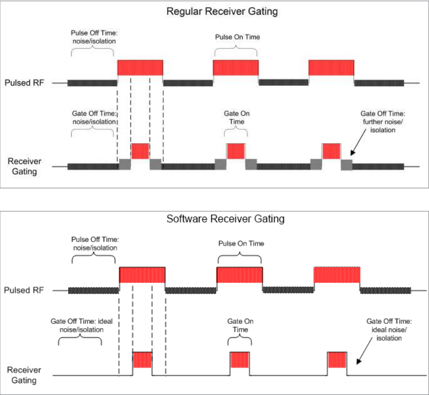
Figure 19. Software gating replaces the residual noise with ideal zeros and increases the receiver sensitivity
