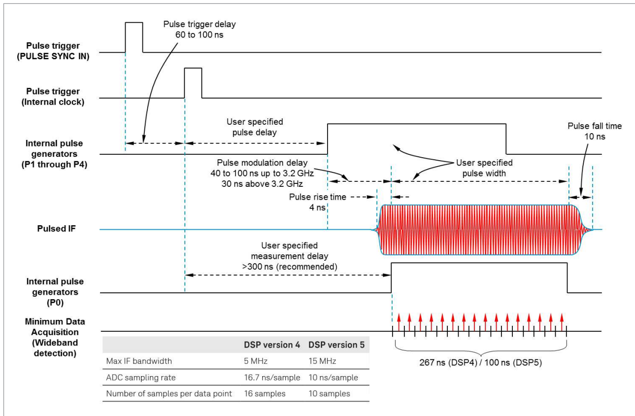
Figure 9. PNA-X pulse system delays with wideband data acquisition
