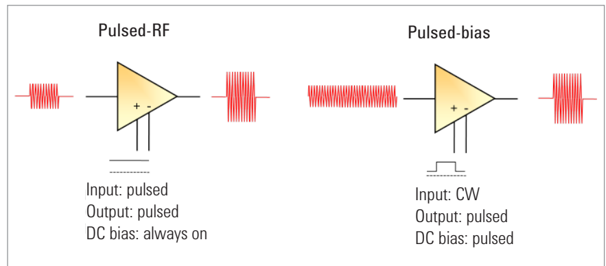
Figure 1. Pulsed-RF and pulsed-bias operation modes
