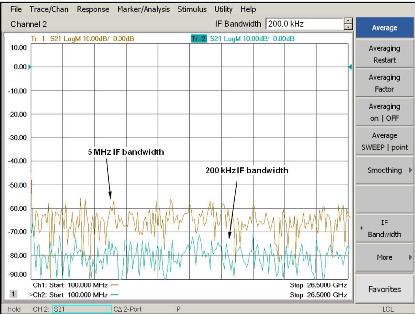
Figure 16. PNA-X wideband pulse measurement dynamic range
