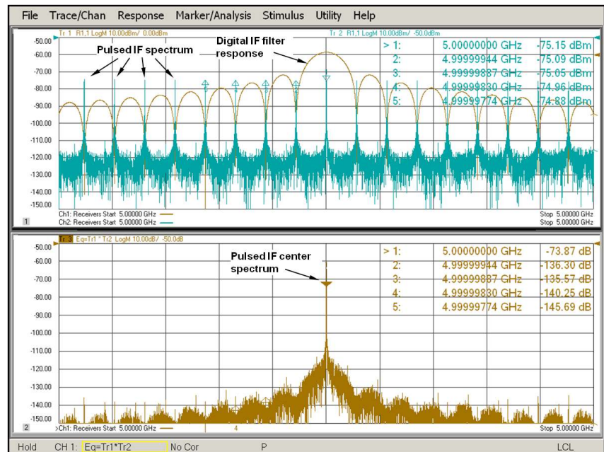
Figure 21. Filter nulling is used to reject undesired pulse spectrum
