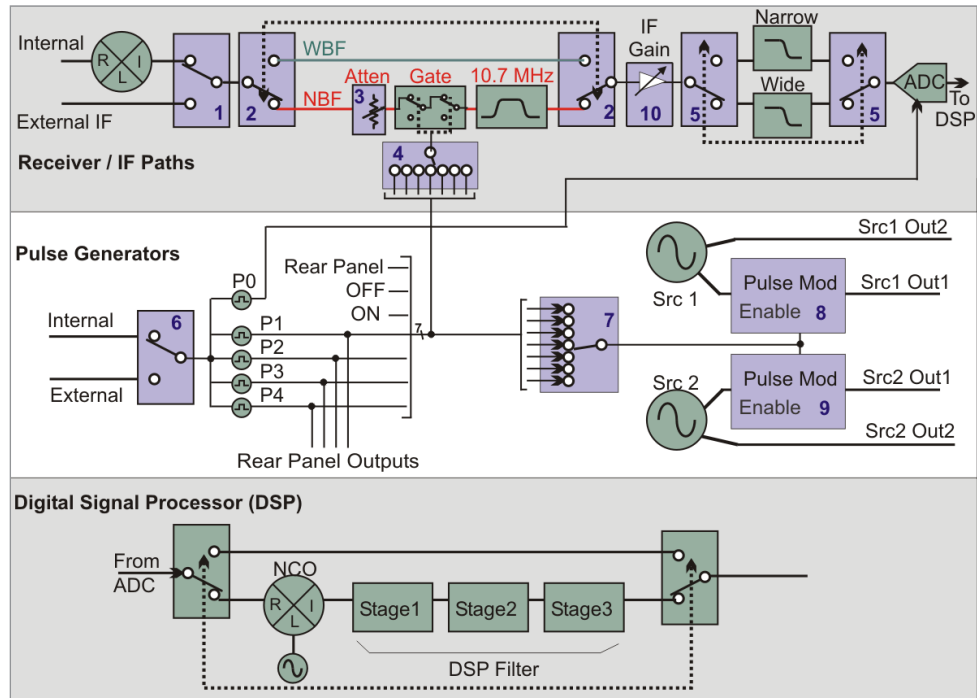
Figure 7. PNA-X IF path block diagram
