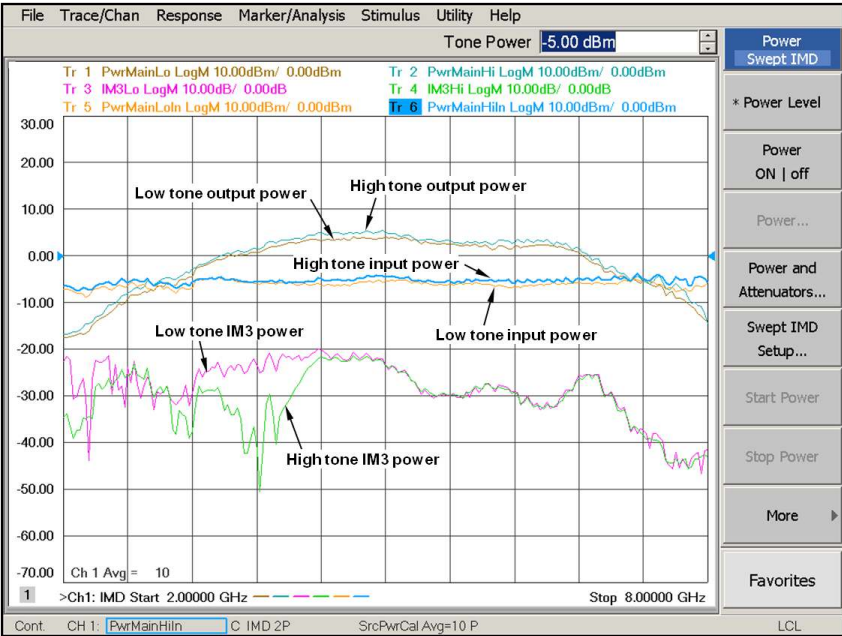
Figure 30a. Wideband pulse swept-frequency IMD measurements with open loop leveling
