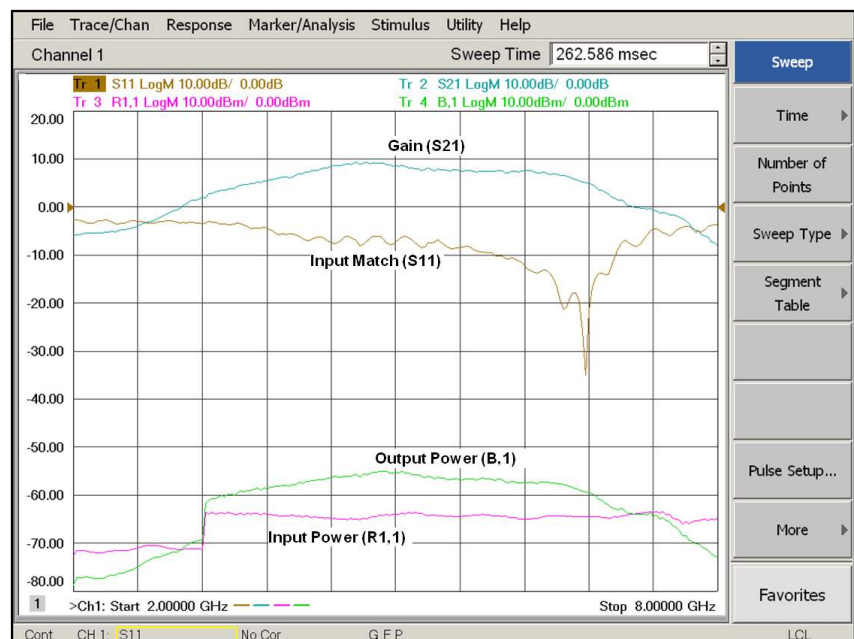
Figure 25a. Uncorrected narrowband pulse measurements
