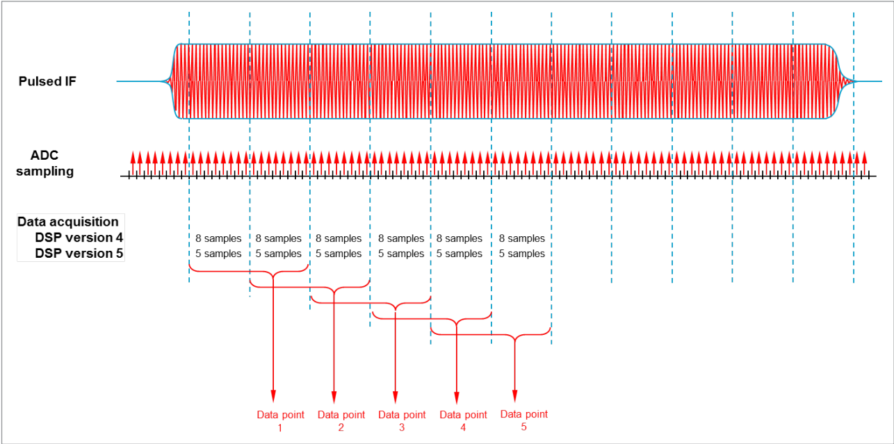
Figure 13. Wideband pulse profile data acquisition using widest IF bandwidth
