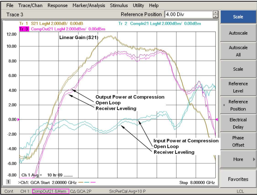
Figure 29. Wideband pulse GCA measurement comparisons between open loop and receiver leveling
