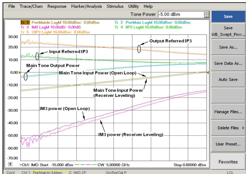
Figure 30c. Wideband pulse swept-power IMD measurement comparisons between open loop and receiver leveling
