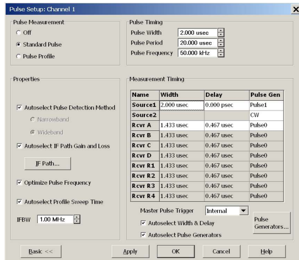
Figure 11b. Advanced Pulse Setup dialog box
