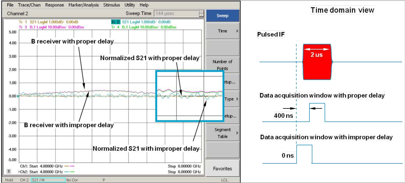
Figure 14b. Measurement errors caused by improper measurement delay
