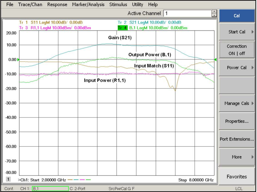
Figure 25b. Measurements after calibration with pulse modulator off
