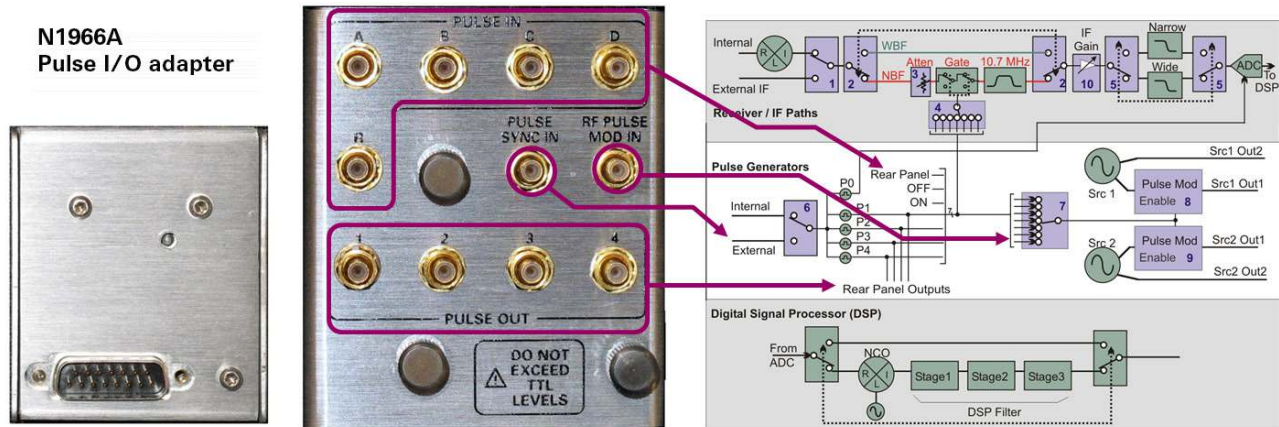
Figure 8. Rear panel pulse I/O
