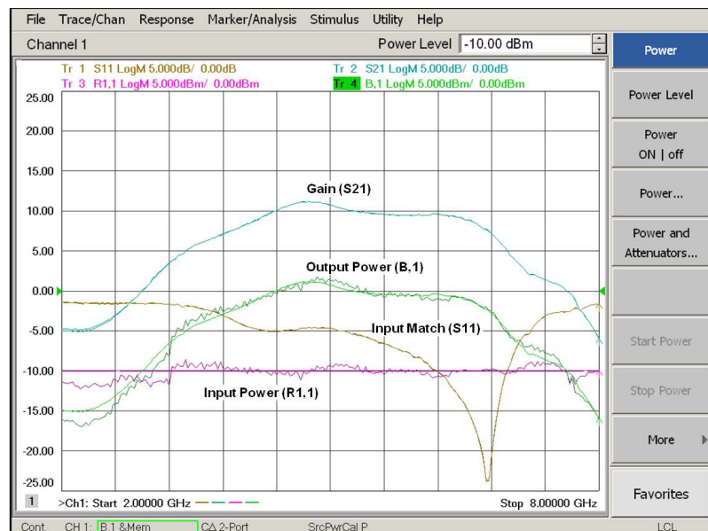
Figure 24. Calibrated wideband pulsed S-parameters and absolute power measurements with a comparison between open loop and receiver leveling modes
