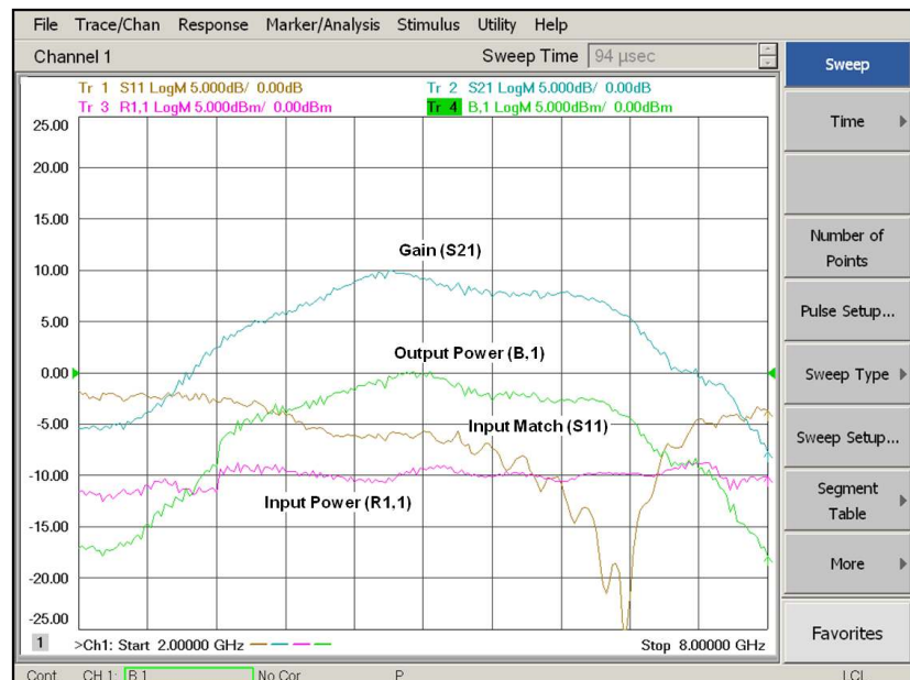
Figure 23. Uncorrected pulsed-RF S-parameters and absolute power measurements using wideband detection
