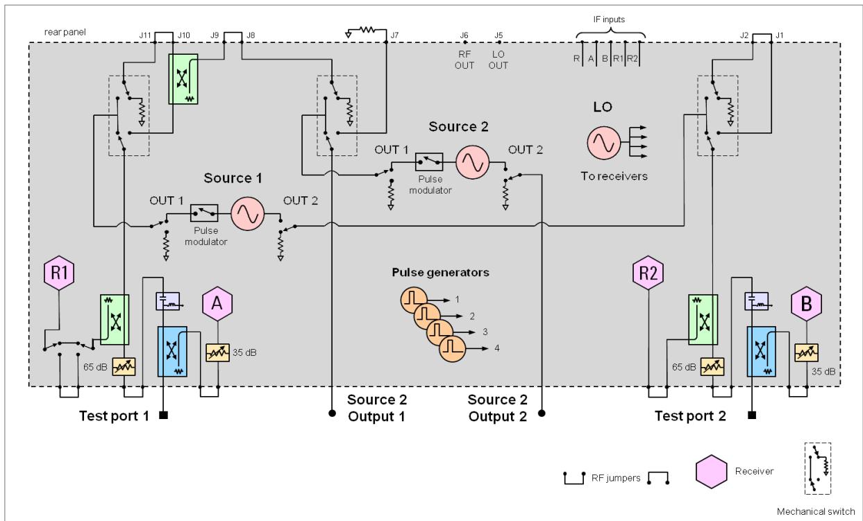
Figure 6. 13.5/26.5 GHz PNA-X block diagram with options 200, 219, 224, 020, 021, 022 and 025
