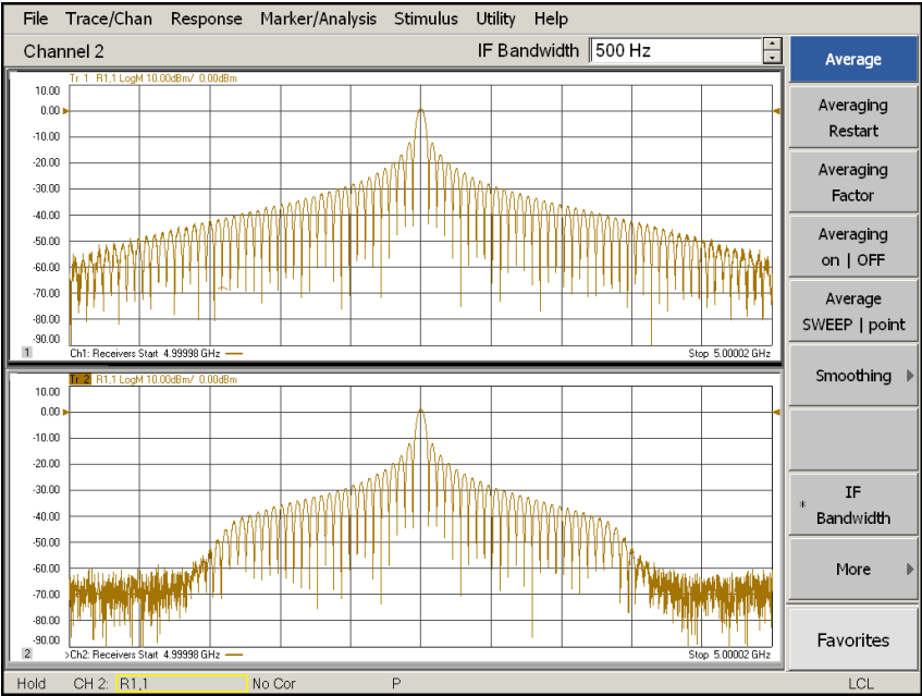
Figure 18. Pulsed-RF signal filtered in wideband IF path and narrowband filter
