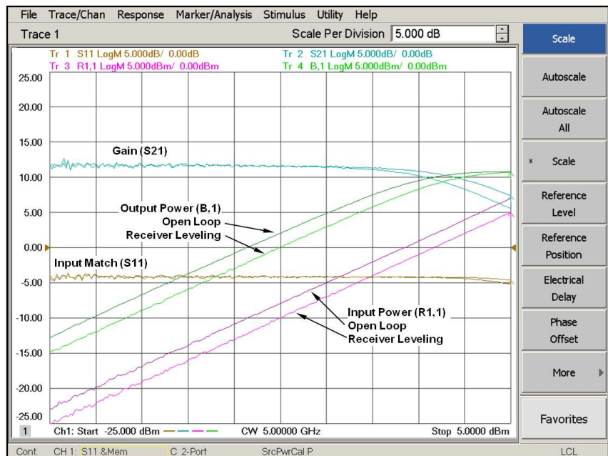
Figure 26. Wideband pulse swept-power measurement comparisons between open loop and receiver leveling modes (calibrated)
