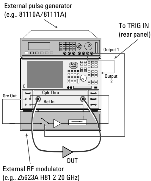
Figure 16. Typical PNA hardware setup for wideband detection
