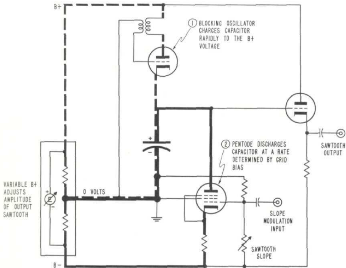
Figure 1. Simplified schematic diagram of a Sawtooth Generator having independent amplitude and slope functions.
