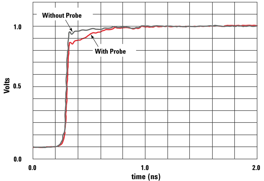
Figure 5. Probes load the circuit at high frequencies and increase the time to drive the circuit to full voltage.
