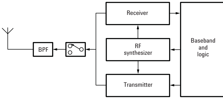
Figure 7. Block diagram of Bluetooth device.
