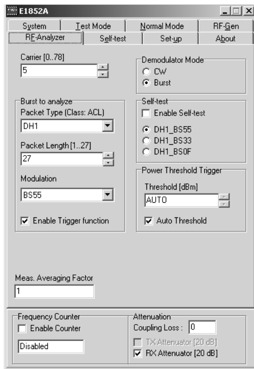
Figure 14. Agilent E1852A display showing “RF-Analyzer” menu and a list of measurement parameters you get by using this menu.
