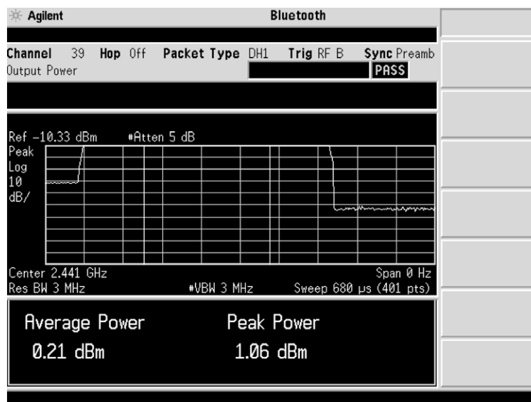
Figure 14. Agilent ESA-E series spectrum analyzer display of peak and average power measurement using the Bluetooth personality (Device setup: CF=2.441 GHz, sweep time 680 \mu s, triggering on IF ch39)
