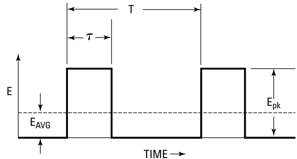
Figure 3. Basic characteristics of a pulsed waveform
