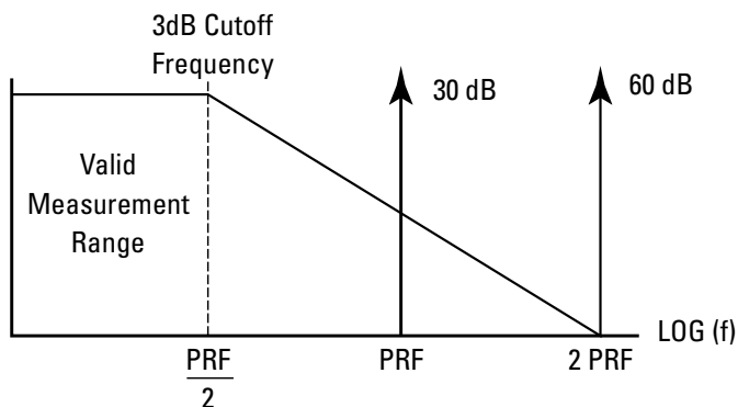
Figure 25. PRF filter response characteristics
