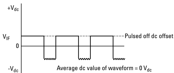
Figure 16. Compensating for dc offset by adjusting \Delta\phi_{LO-RF} to produce an average dc value of 0 Vdc
