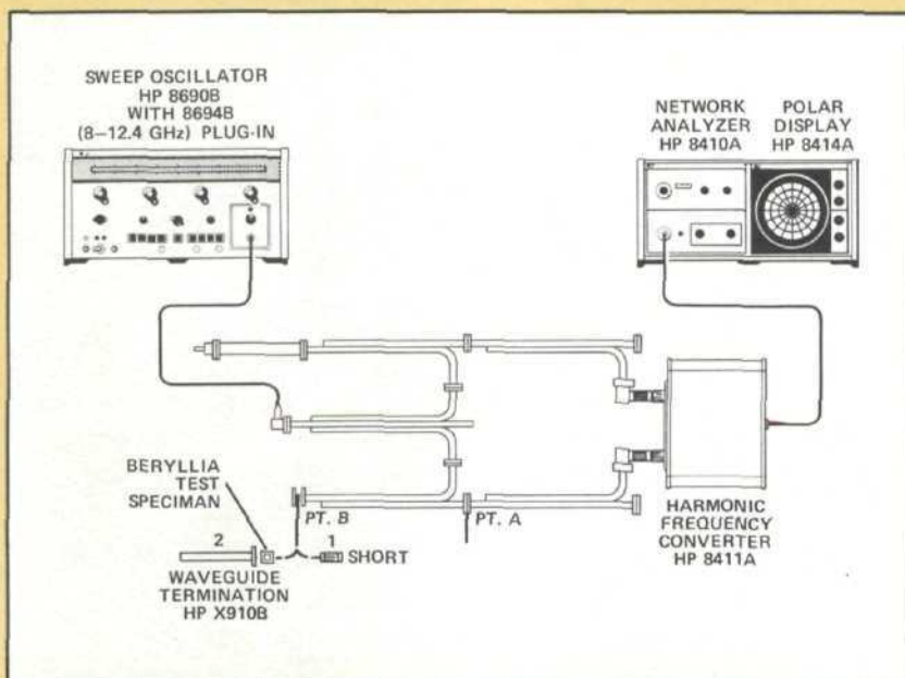
Figure 7-6. Equipment Setup
