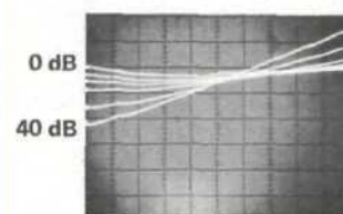
25°/DIV SWEEP 0.1 - 1.8 GHz
