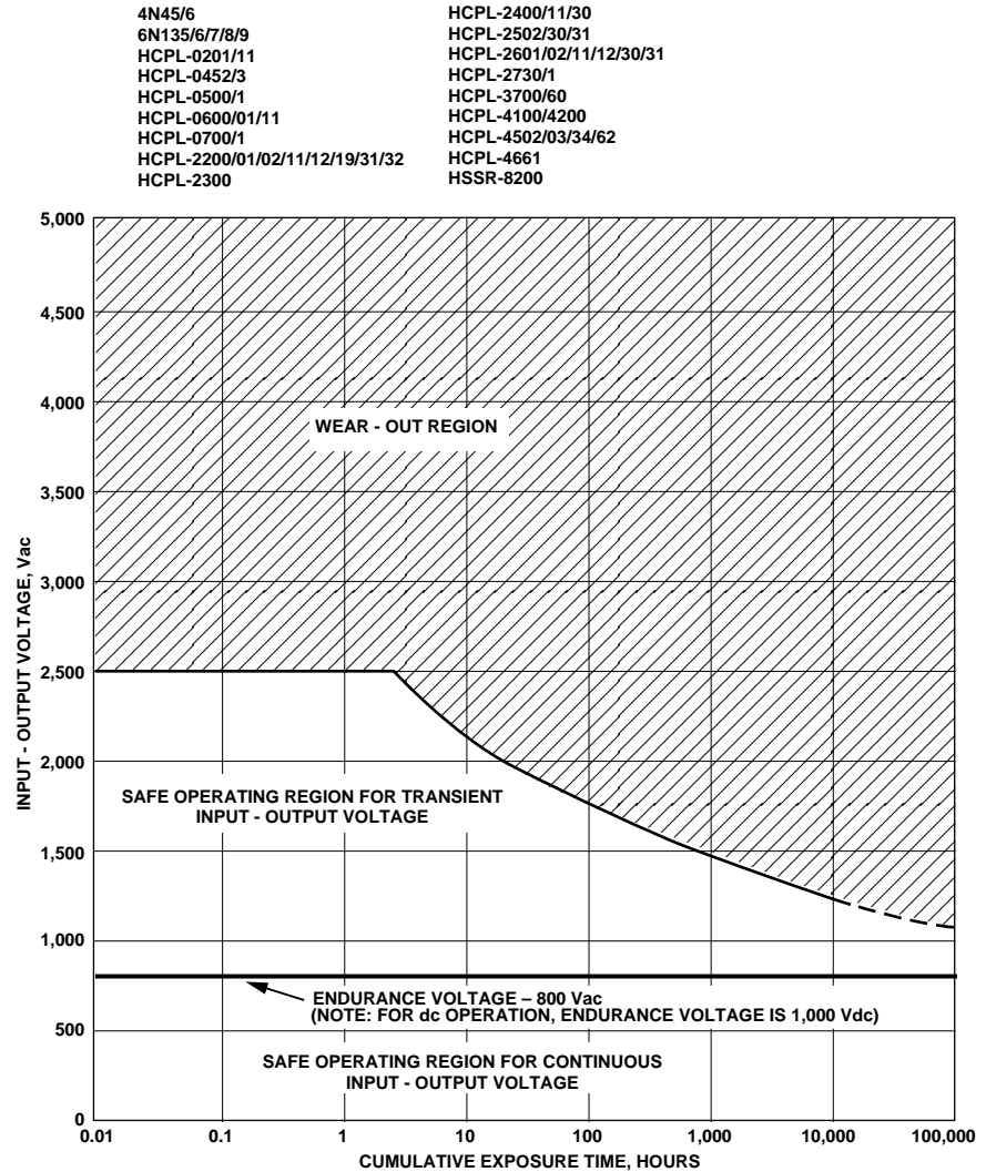
Figure 1. Recommended Safe Operating Area for Input-Output Voltage-Endurance Voltage for Category 1 Optocouplers.
