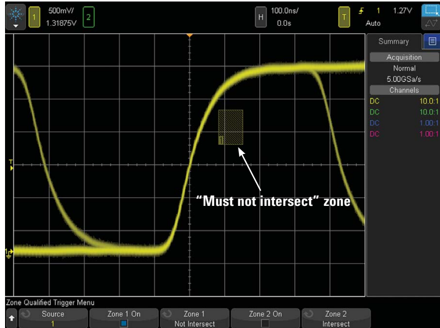
Figure 3: Capturing and displaying just waveforms with “normal” edges using InfiniiScan Zone Trigger.
