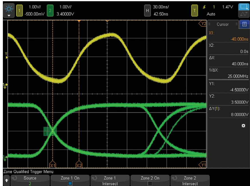
Figure 6: Using InfiniiScan Zone Trigger to isolate valid setup times.
