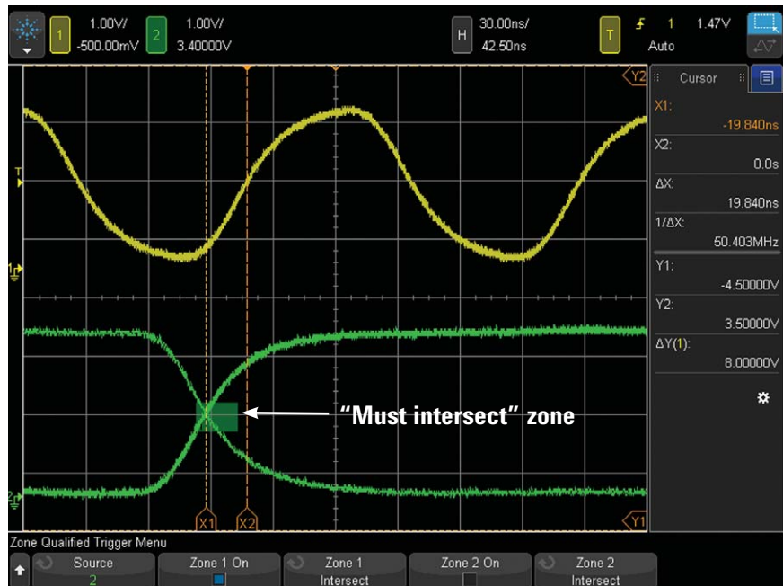
Figure 5: Using InfiniiScan Zone Trigger to isolate setup time violations.
