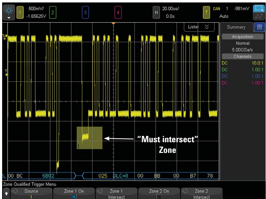
Figure 11: Using InfiniiScan Zone Trigger to synchronize on just frames that include arbitration.
