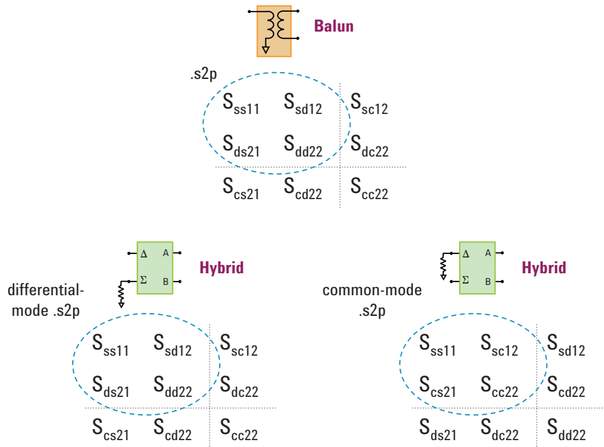
Figure 36. Choose appropriate four differential- or common-mode parameters
