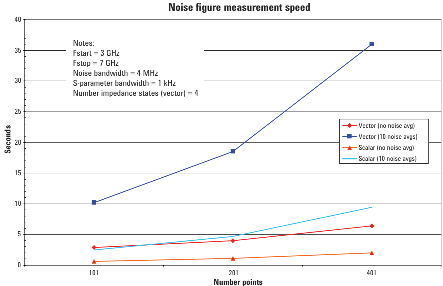
Figure 25. Scalar noise calibration offers about a four times improvement in measurement speed
