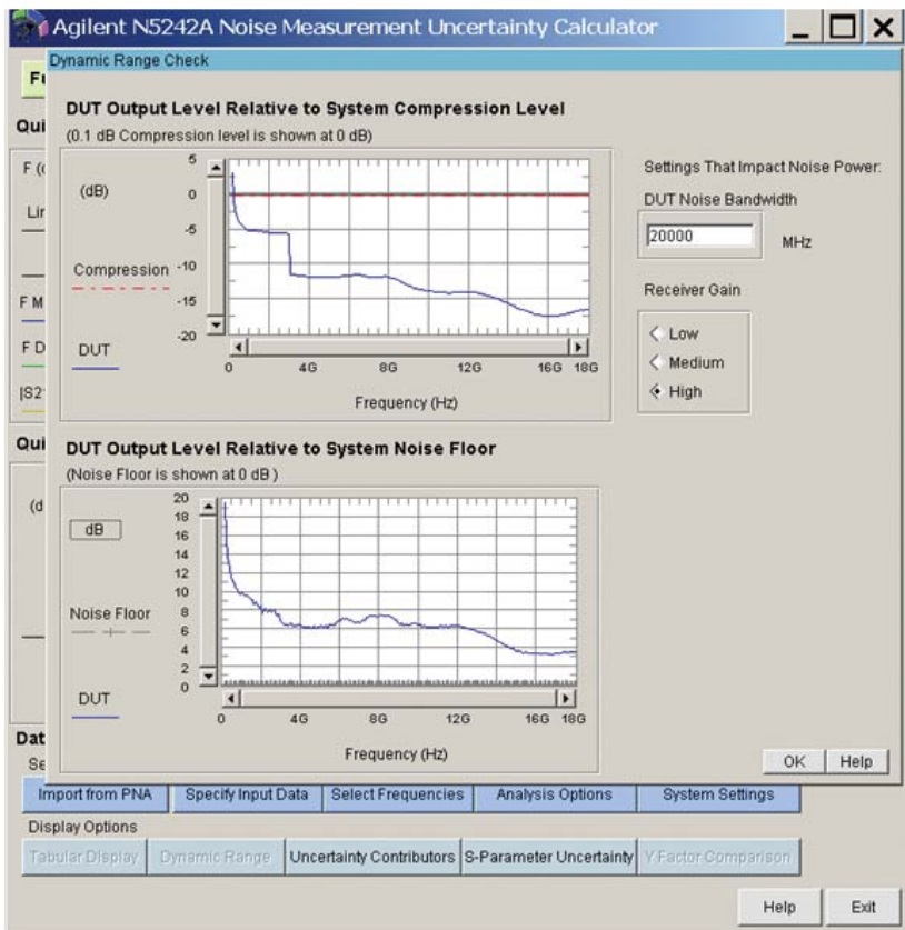
Figure 49. Agilent's PNA-X noise figure uncertainty calculator shows if the DUT's noise power is causing compression in the noise receiver.
