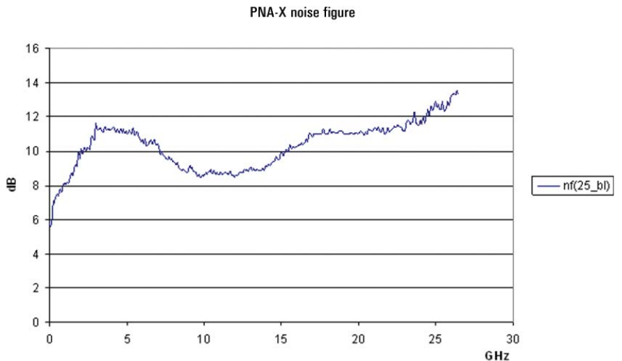
Figure 28. Typical noise figure of port two
