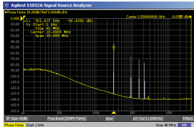
Figure 28. The phase noise of a clock signal in the phase-noise frequency domain
