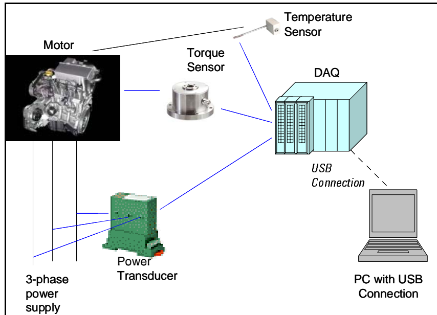
Figure 2 Measurement setup using Agilent's USB DAQ device
