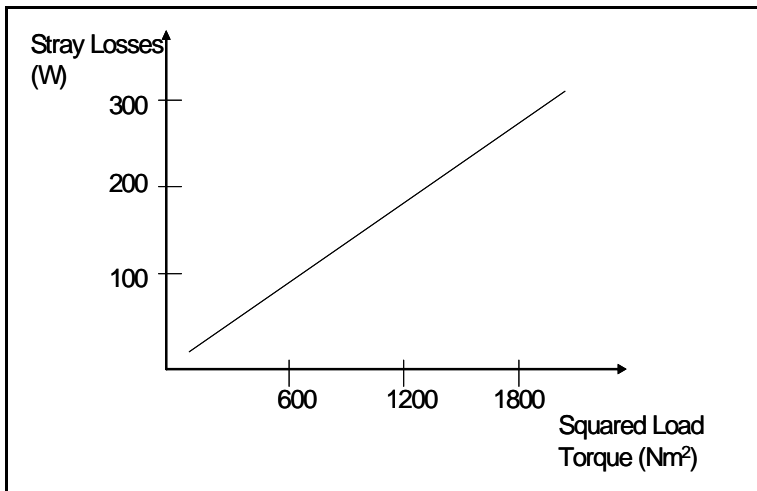
Figure 1 Graph of squared load torque versus stray loss
