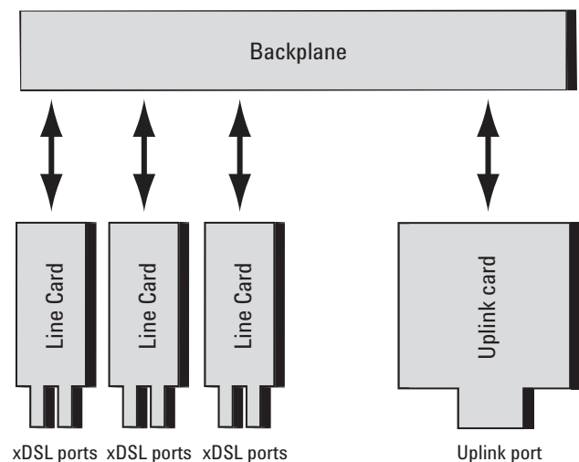
High-level DSLAM Architecture Diagram
