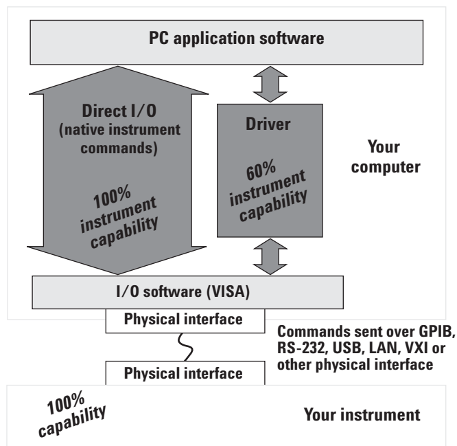
Figure 4. I/O software layer
