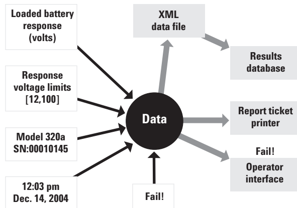
Figure 5. Overview of data collection process
