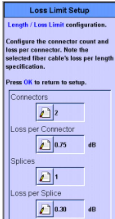
Figure 0: WireScope 350 set-up screen for specifying the loss budget per TIA and ISO standards.
