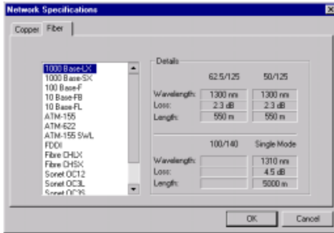
Figure 1: An example of fiber optic network test limits programmed into a field tester.
