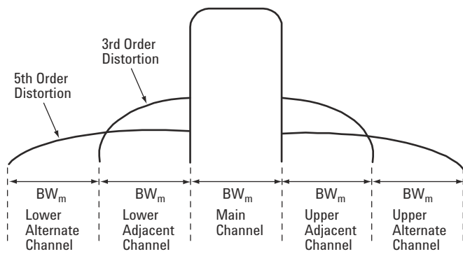
Figure 3-3b Spectral Regrowth as Displayed on the Log Scale
