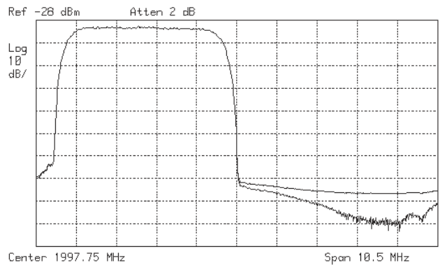
Figure 5-3 W-CDMA Signal with and without Noise Subtraction
