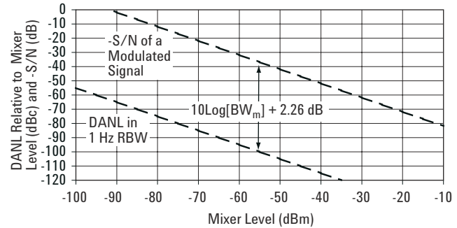
Figure 3-2 S/N vs. Mixer Level for Digitally Modulated Signals
