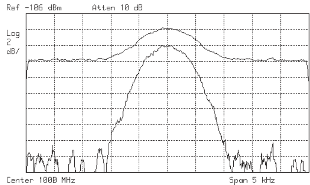
Figure 5-2 CW Signal with and without Noise Subtraction
