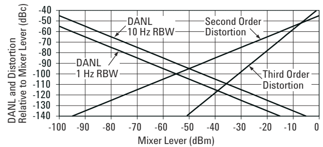
Figure 2-10 Dynamic Range Chart
