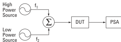
Figure 1-4 Two-Tone Gain Compression Measurement Setup
