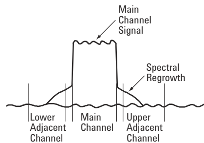
Figure 1–5 Spectral Regrowth of a Digitally Modulated Signal
