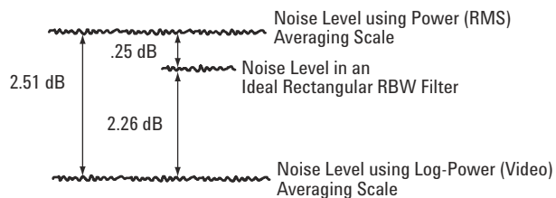
Figure 2-4 Averaging Scale Effect on Displayed Noise
