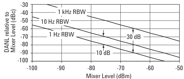
Figure 2-3 Noise Floor with Different RBW Settings
