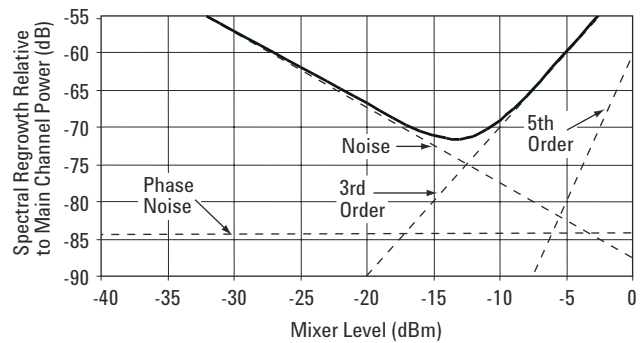
Figure 3-7 Dynamic Range Chart for W-CDMA
