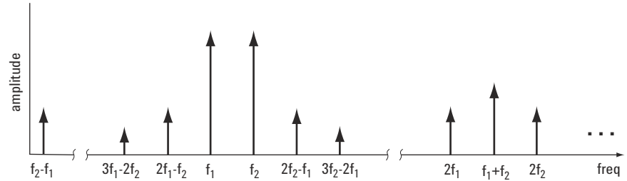
Figure 1-2 Two-Tone Intermodulation Distortion
