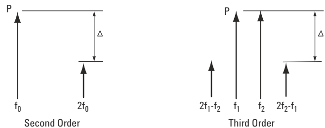
Figure 2-8 Second and Third Order Distortion Spectrum
