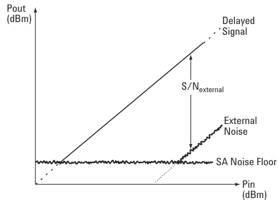
Figure 2-5 SA Pout vs. Pin with External Noise
