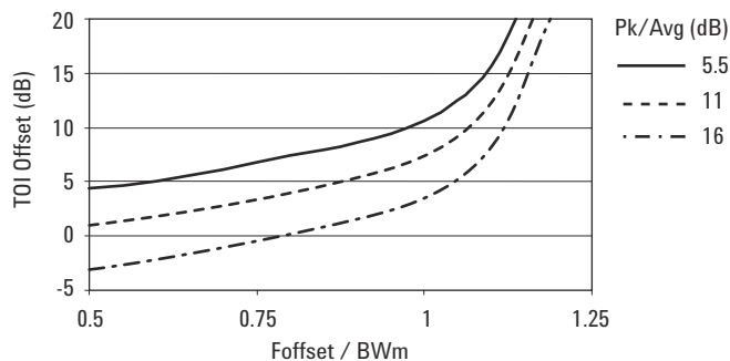
Figure 3-4 Effective TOI of Digitally Modulated Signal versus Frequency Offset from Main Channel
