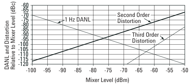
Figure 4-3 Dynamic Range Chart with the Internal Preamp Selected
