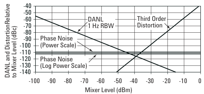
Figure 2-12 Phase Noise Represented on the Dynamic Range Chart
