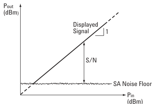
Figure 2-1 Spectrum Analyzer Pout vs. Pin Characteristic
