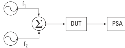
Figure 1-3 Two-Tone Intermodulation Distortion Measurement Setup
