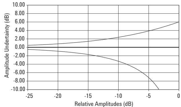
Figure 2-17 Amplitude Uncertainty due to Two Coherent CW Tone Adding Together
