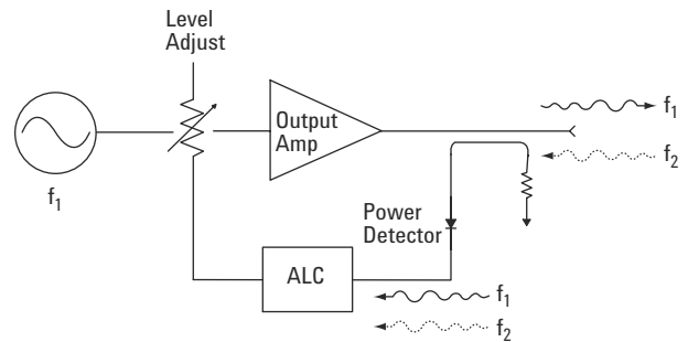
Figure 5-1 Simplified Output Section of a Signal Generator
