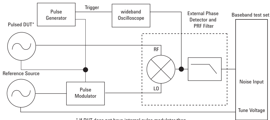
Figure 27. Recommended hardware configuration for pulsed absolute measurements when a PRF filter is required
