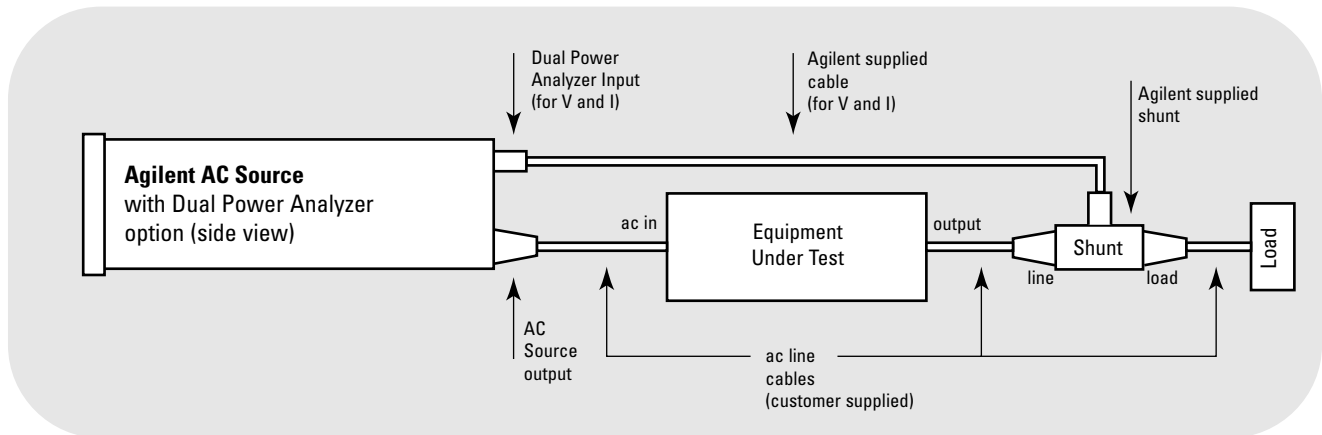
Figure 5. UPS test configuration using Agilent ac source with Dual Power Analyzer option
