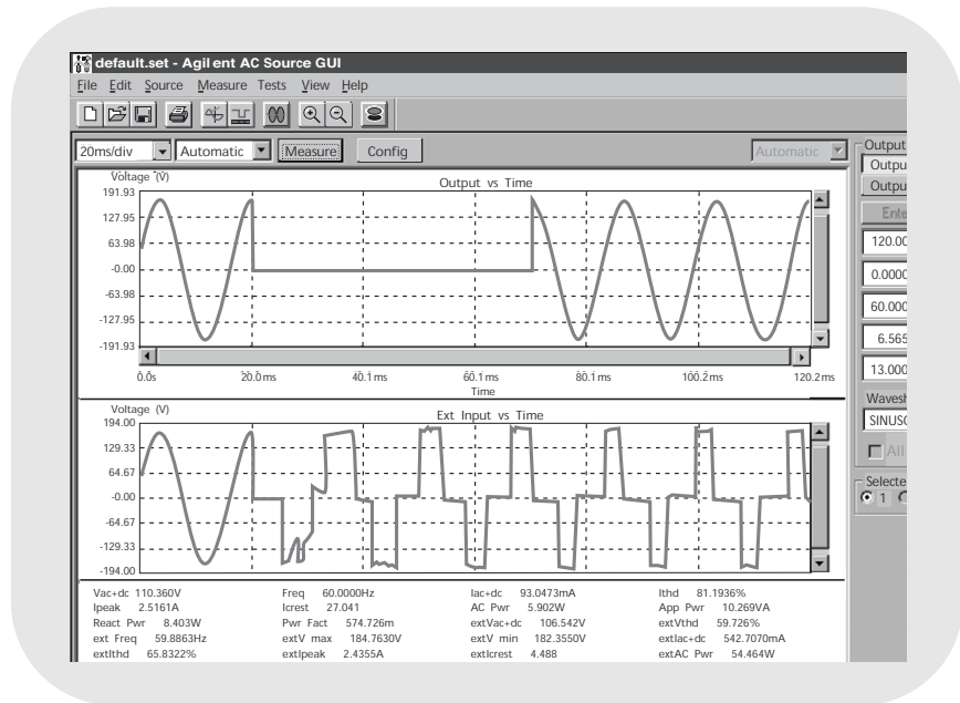
Figure 6. GUI screen-shot of waveforms using Agilent ac source with Dual Power Analyzer option. Top waveform is ac source output voltage (UPS input voltage). Bottom waveform is UPS output voltage. Note that all measured waveform data shown here is read directly from the ac source; no external instruments are used to read data.
