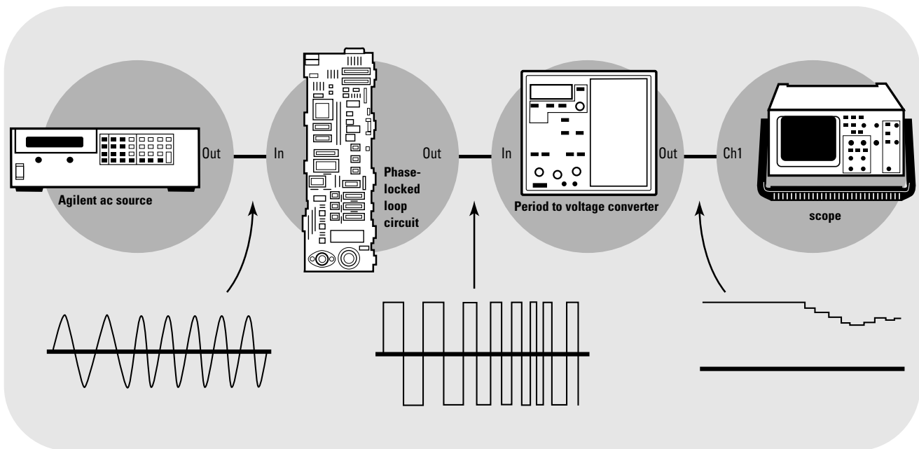
Figure 4. Phase-locked loop response test setup
