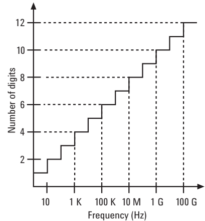
Figure 1. The number of digits displayed by a direct counter versus frequency (for a 1 second gate time).
