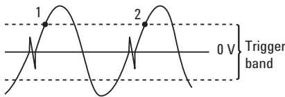
Figure 10. Lowering the trigger sensitivity by expanding the trigger band produces the desired count.
