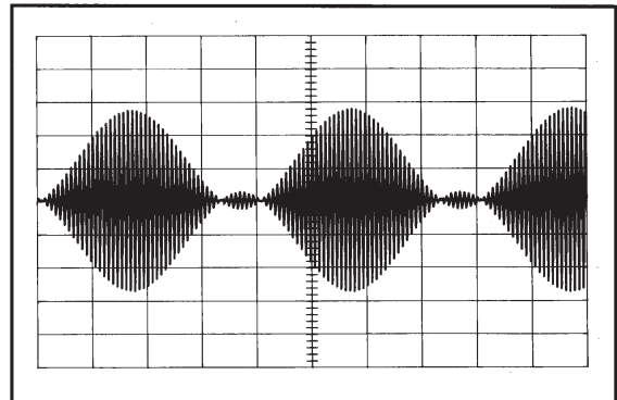
WAVEFORM NAME/DESCRIPTION: AM signal with over 100% negative peak modulation.
