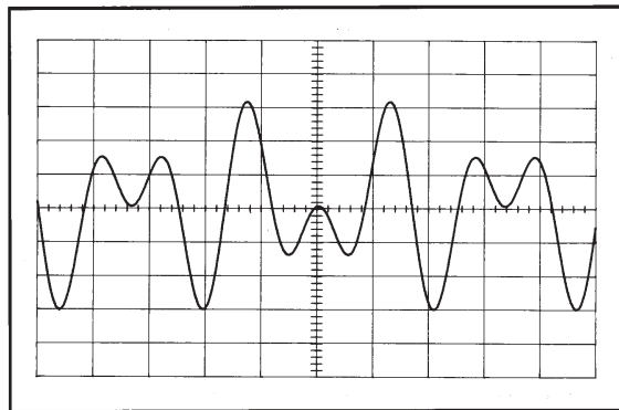
WAVEFORM NAME/DESCRIPTION: ILS two-tone composite signal.
