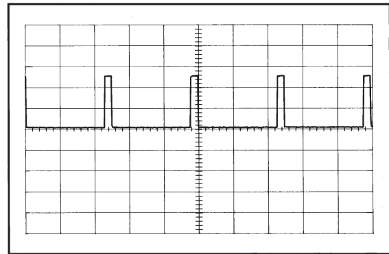
WAVEFORM NAME/DESCRIPTION: Variable duty cycle pulses—duty cycle 0% to 50%.
