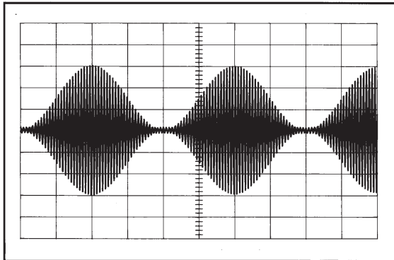
WAVEFORM NAME/DESCRIPTION: Distorted AM due to capacitive coupling of carrier past the AM modulator.
